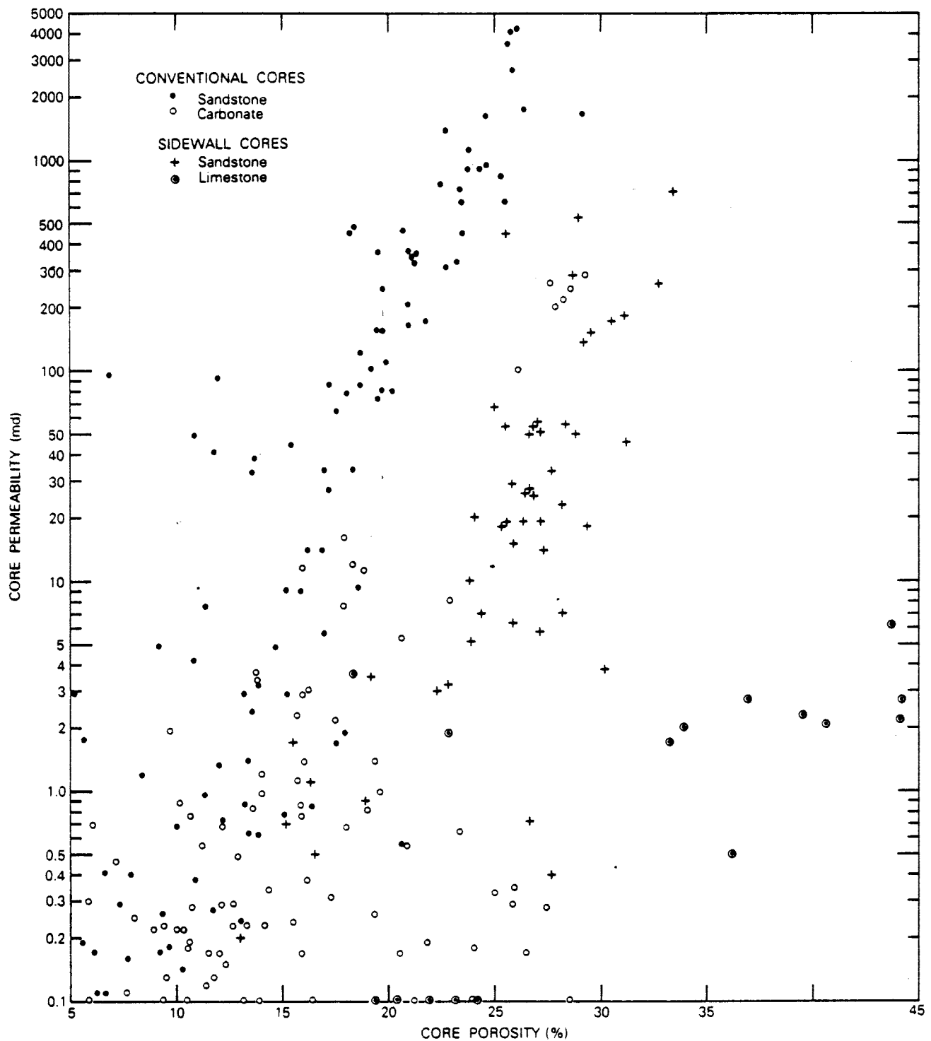
Figure 16. Core porosities plotted against core permeabilities, COST No. GE-1 well
