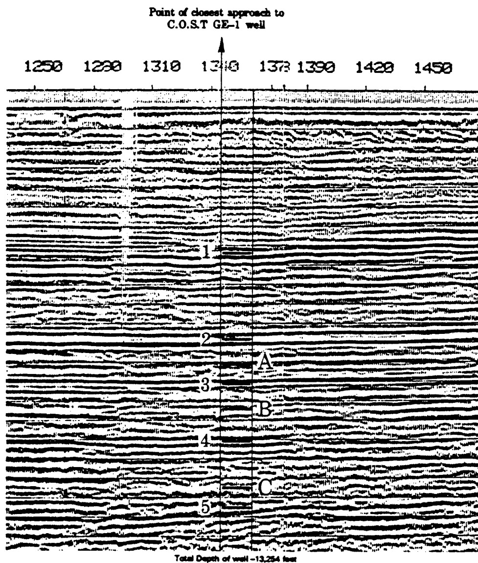
Figure 7. Seismic reflectors recognized within the COST No. GE-1 well
