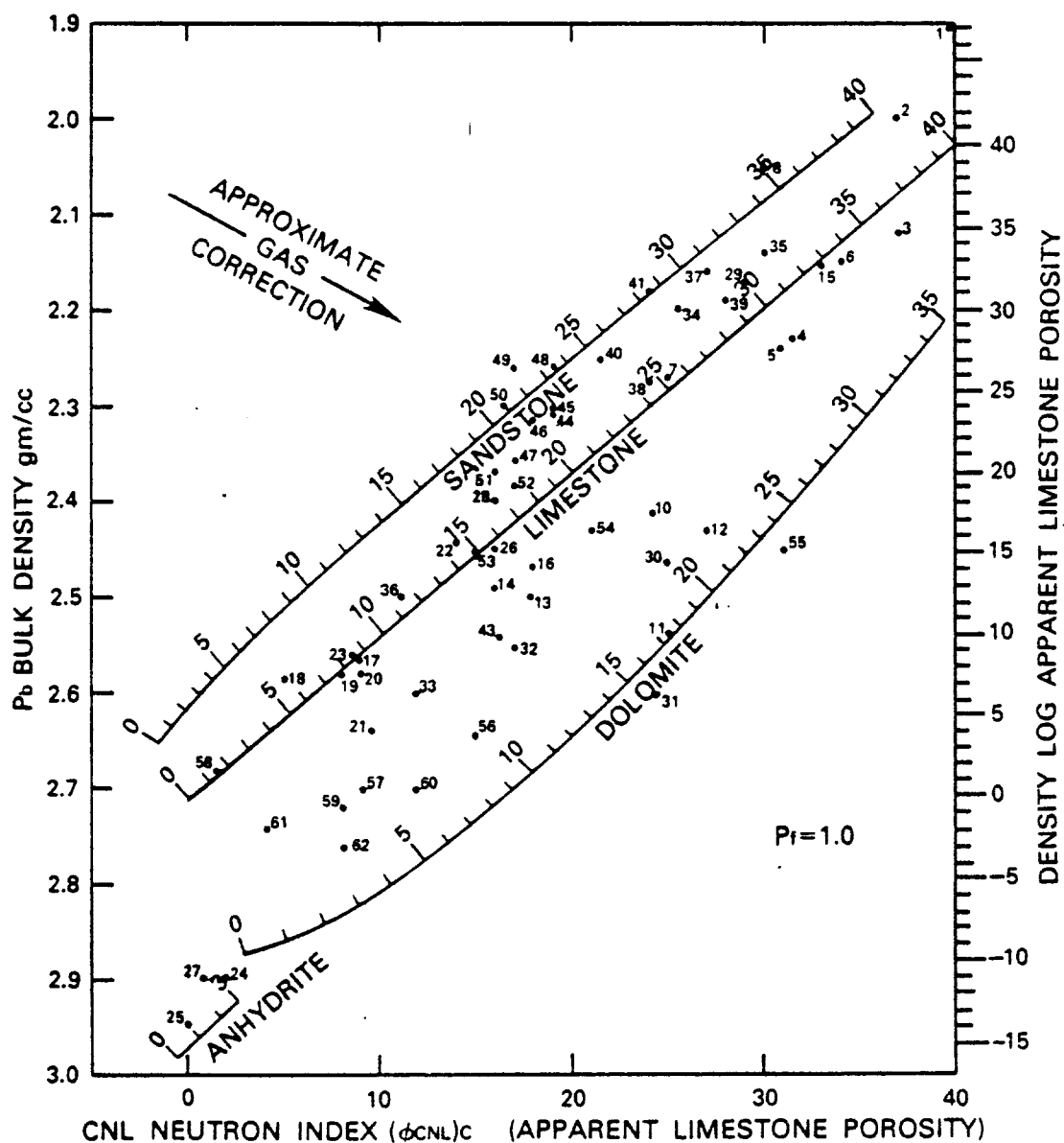
Figure 11. Porosity and lithology determination from Formation Density Log and Compensated Neutron Log (CNL) for fresh-water, liquid-filled holes (form Copyright 1972 by Schlumberger, Ltd.)
