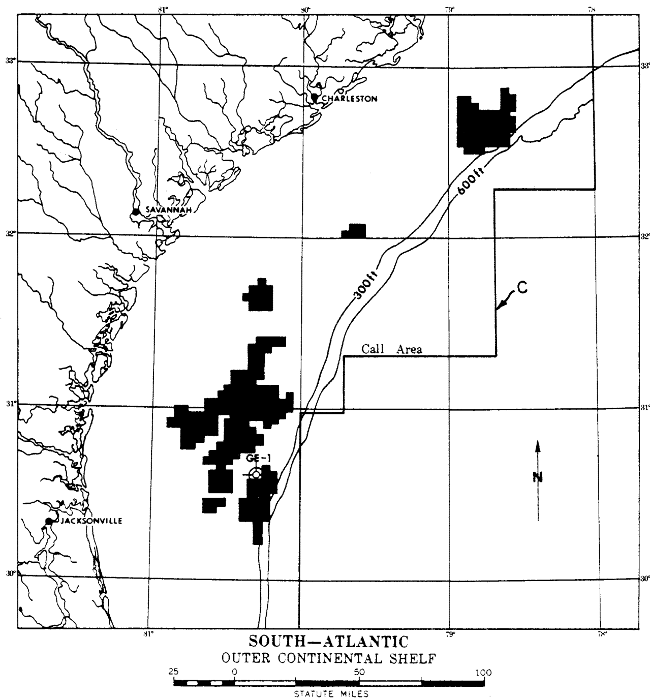
Figure 1. Map of the South Atlantic O.C.S. showing the location of the COST No. GE-1 well, the tracts offered for lease in Sale No. 43 (in black) and the eastern limits of the call area for tract nominations (C).
