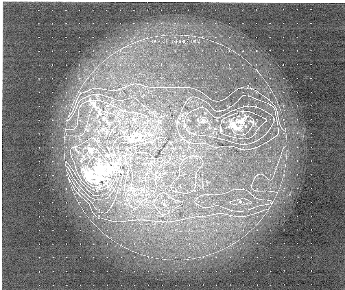
Figure 1. The 3.3-mm solar radio temperature contour map made on 30 June 1971 superposed on a concurrent H \alpha photograph. The contours are labeled in percent enhancement relative to the temperature of the undisturbed regions denoted by the hatched contours.
