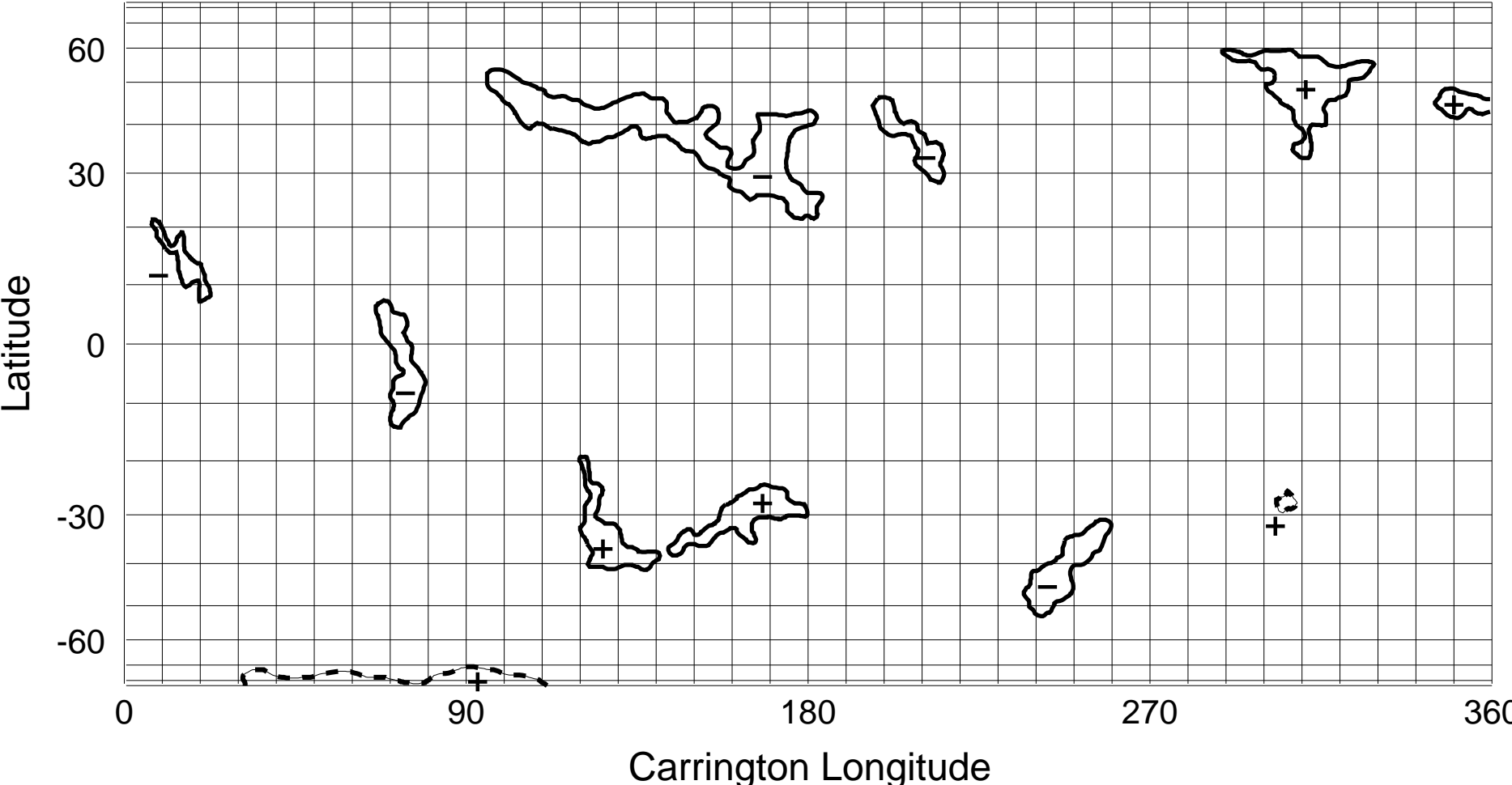
NSO/KP He I 1083 nm Coronal Hole Map: Carrington Rotation 1820
