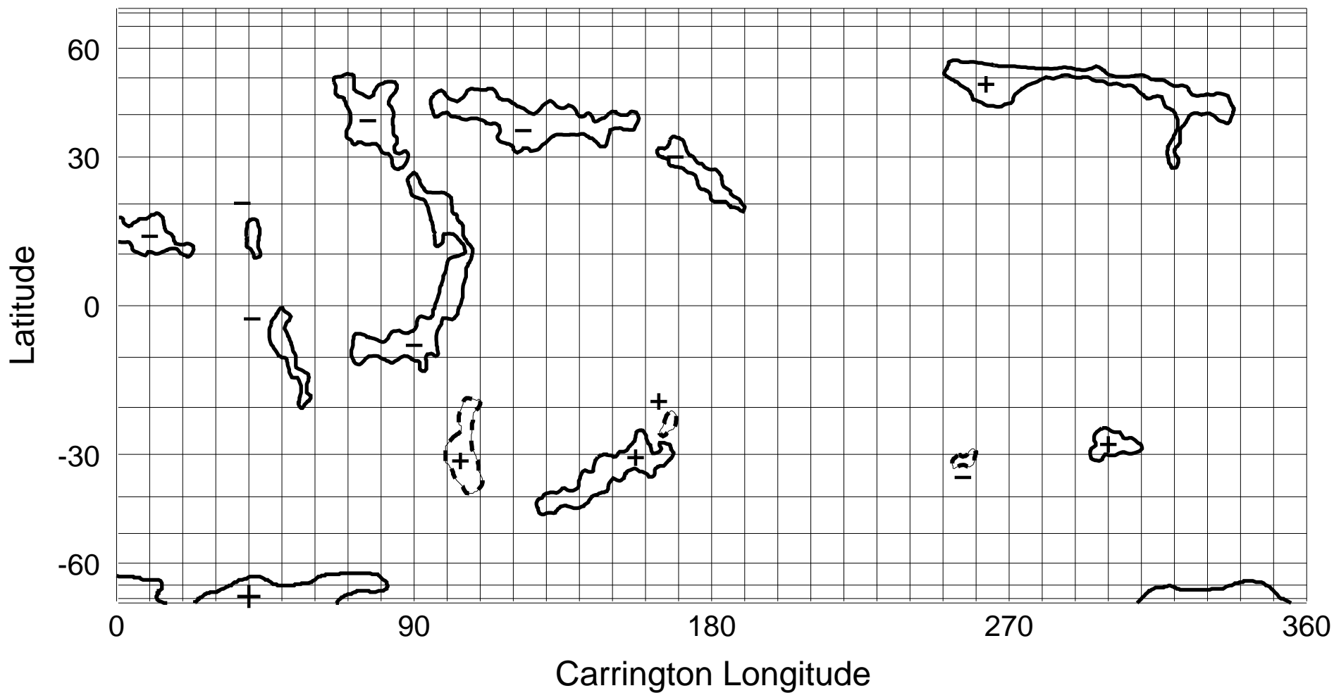
NSO/KP He I 1083 nm Coronal Hole Map: Carrington Rotation 1821
