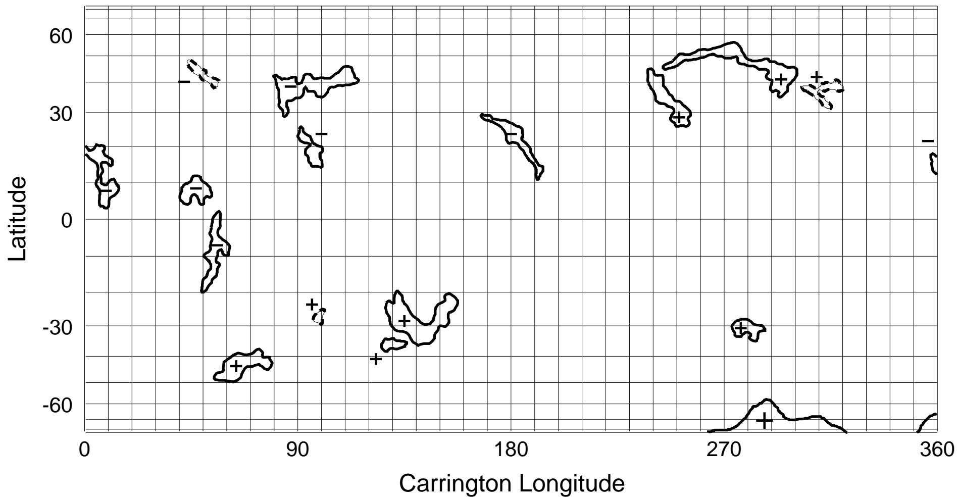
NSO/KP He I 1083 nm Coronal Hole Map: Carrington Rotation 1822
