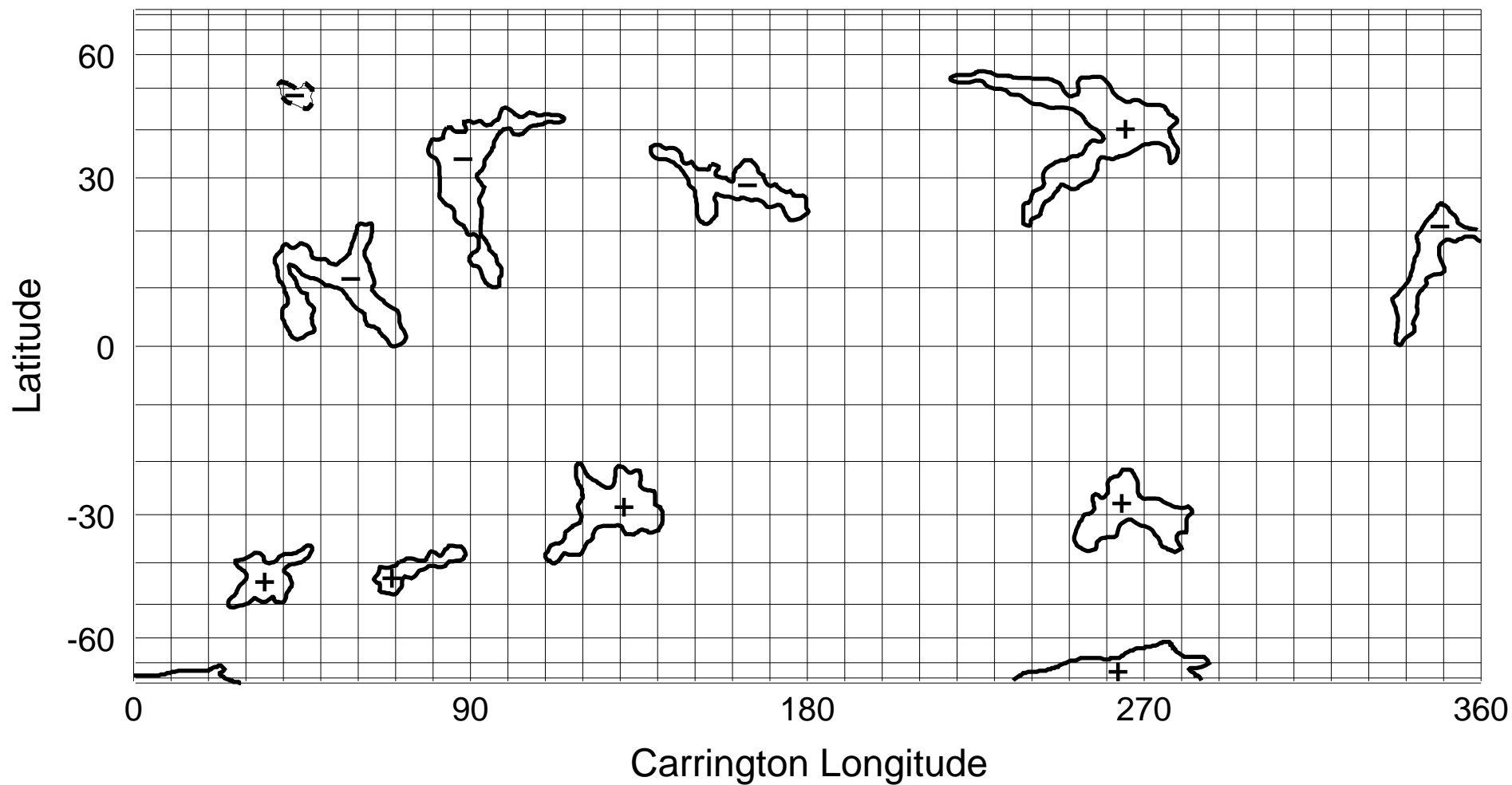
NSO/KP He I 1083 nm Coronal Hole Map: Carrington Rotation 1823
