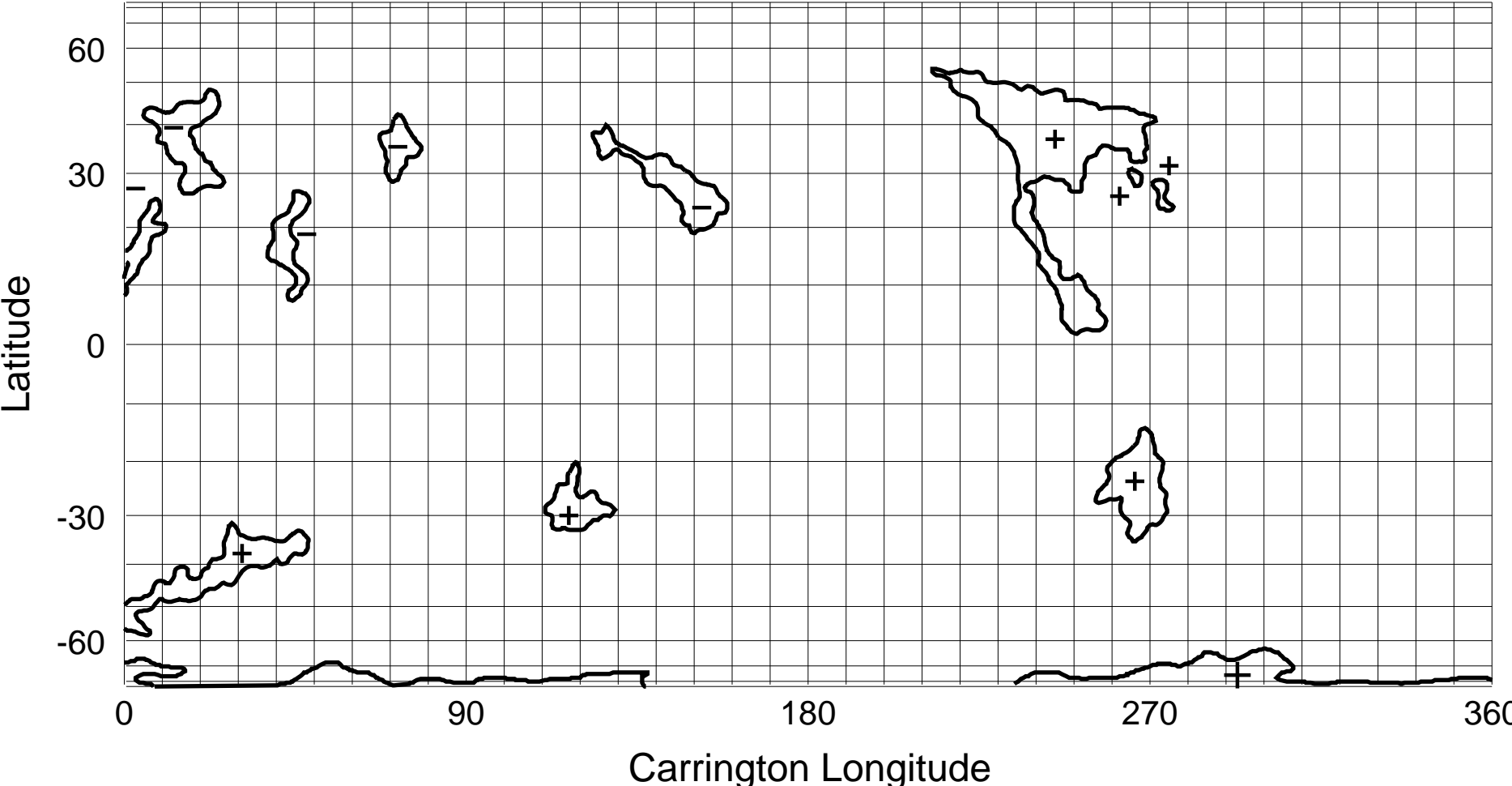
NSO/KP He I 1083 nm Coronal Hole Map: Carrington Rotation 1824
