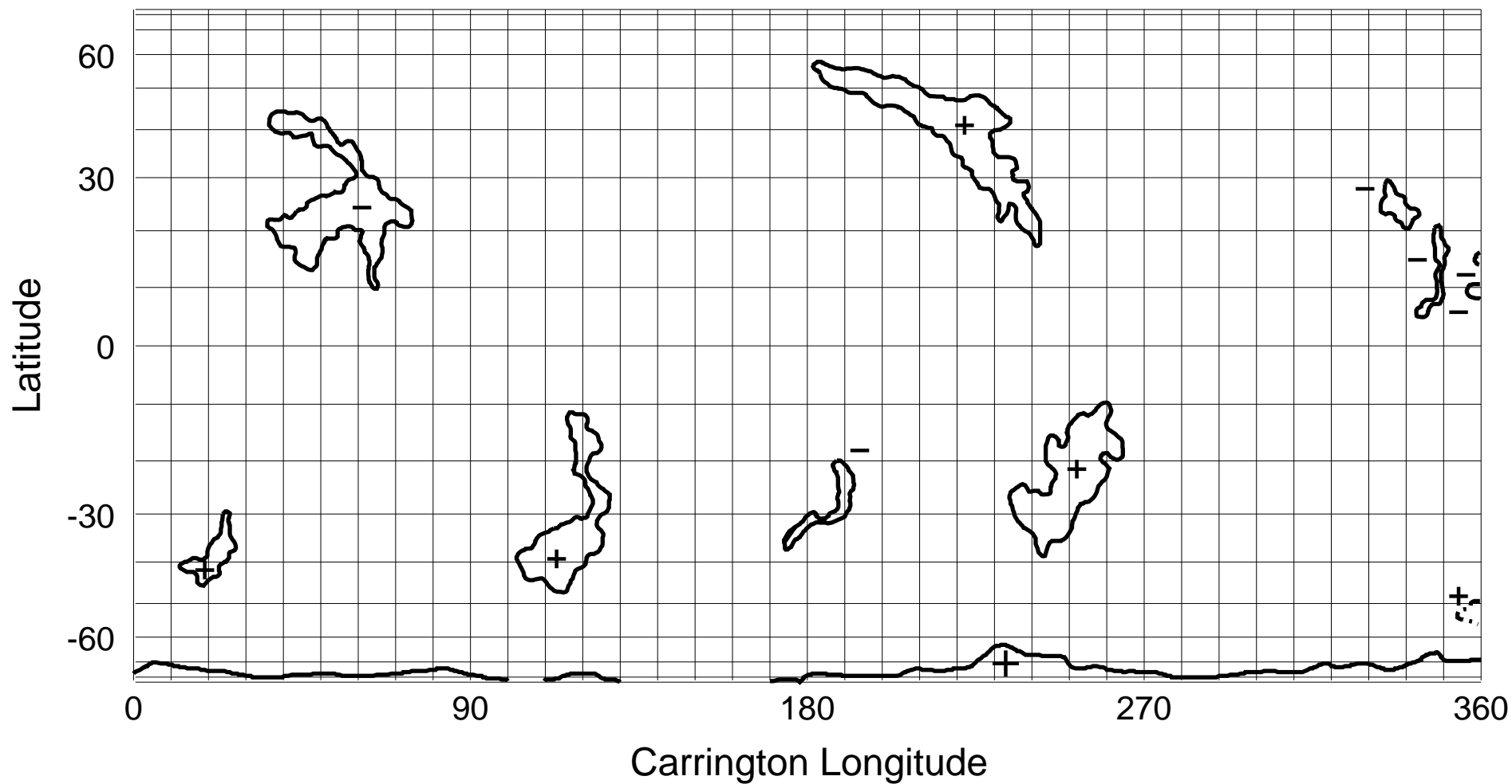
NSO/KP He I 1083 nm Coronal Hole Map: Carrington Rotation 1825
