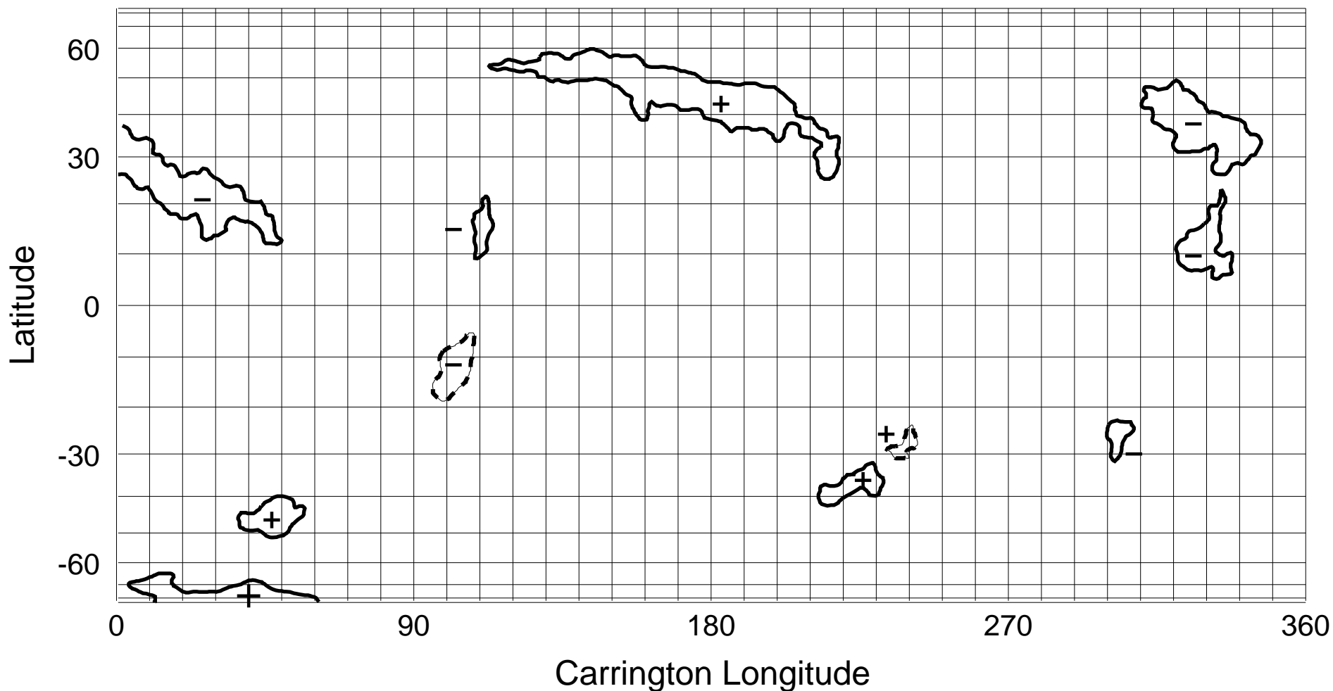
NSO/KP He I 1083 nm Coronal Hole Map: Carrington Rotation 1827
