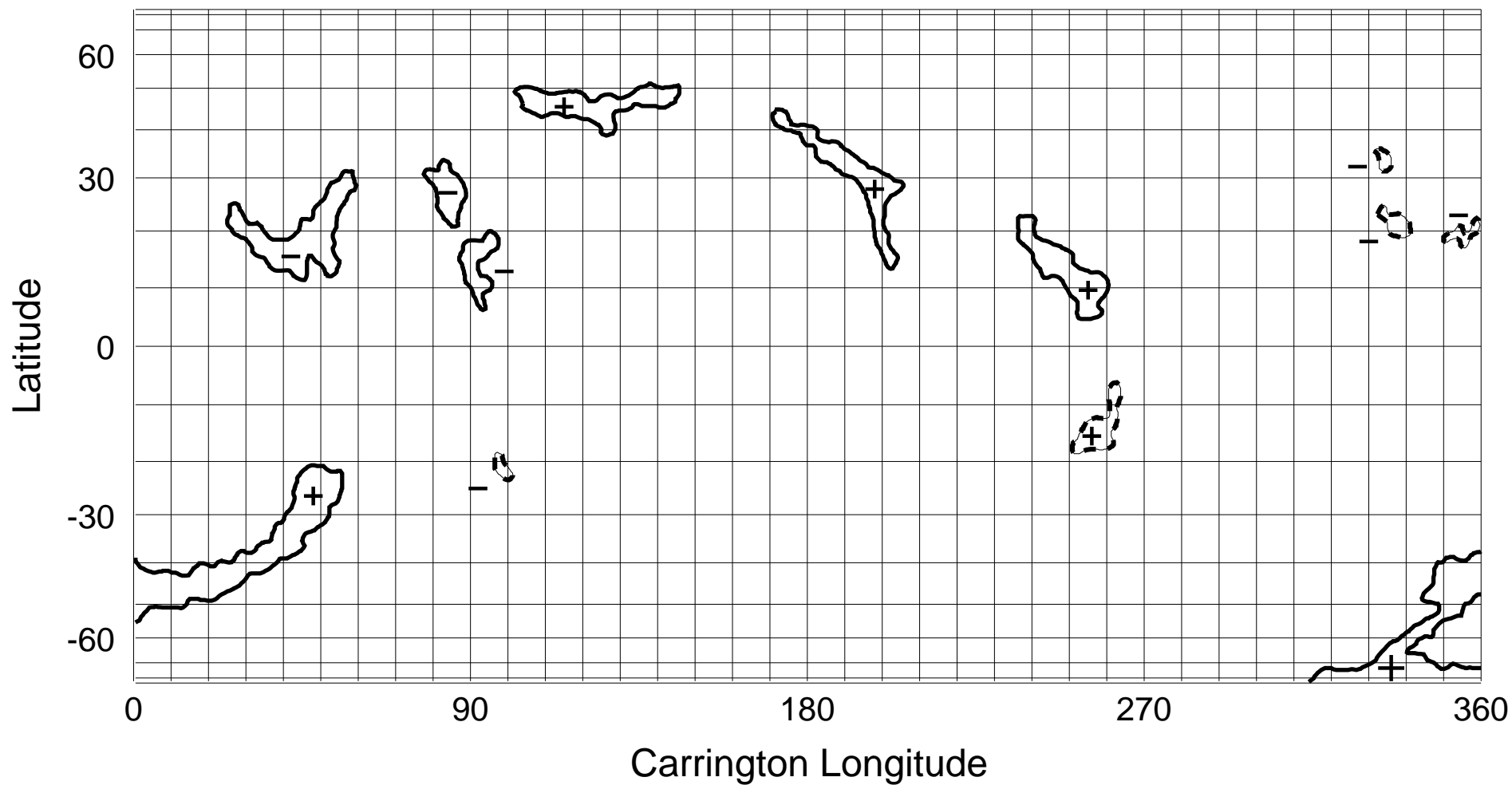
NSO/KP He I 1083 nm Coronal Hole Map: Carrington Rotation 1829
