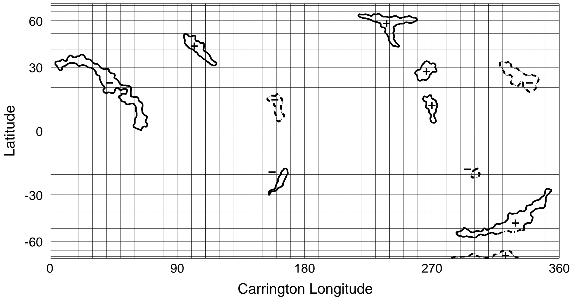
NSO/KP He I 1083 nm Coronal Hole Map: Carrington Rotation 1831
