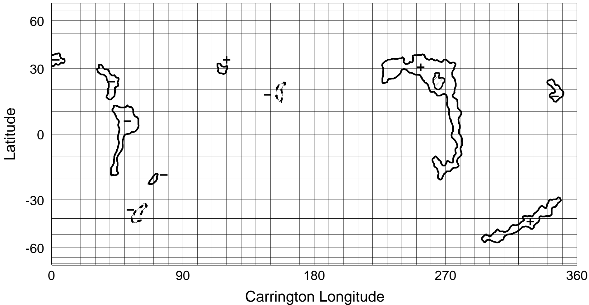
NSO/KP He I 1083 nm Coronal Hole Map: Carrington Rotation 1832
