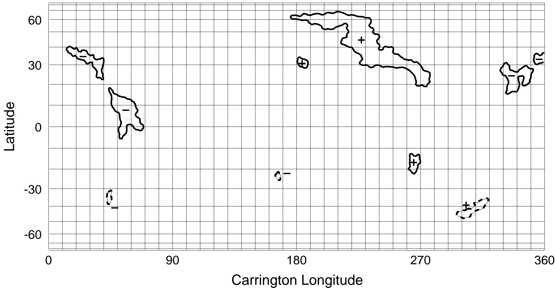
NSO/KP He I 1083 nm Coronal Hole Map: Carrington Rotation 1833
