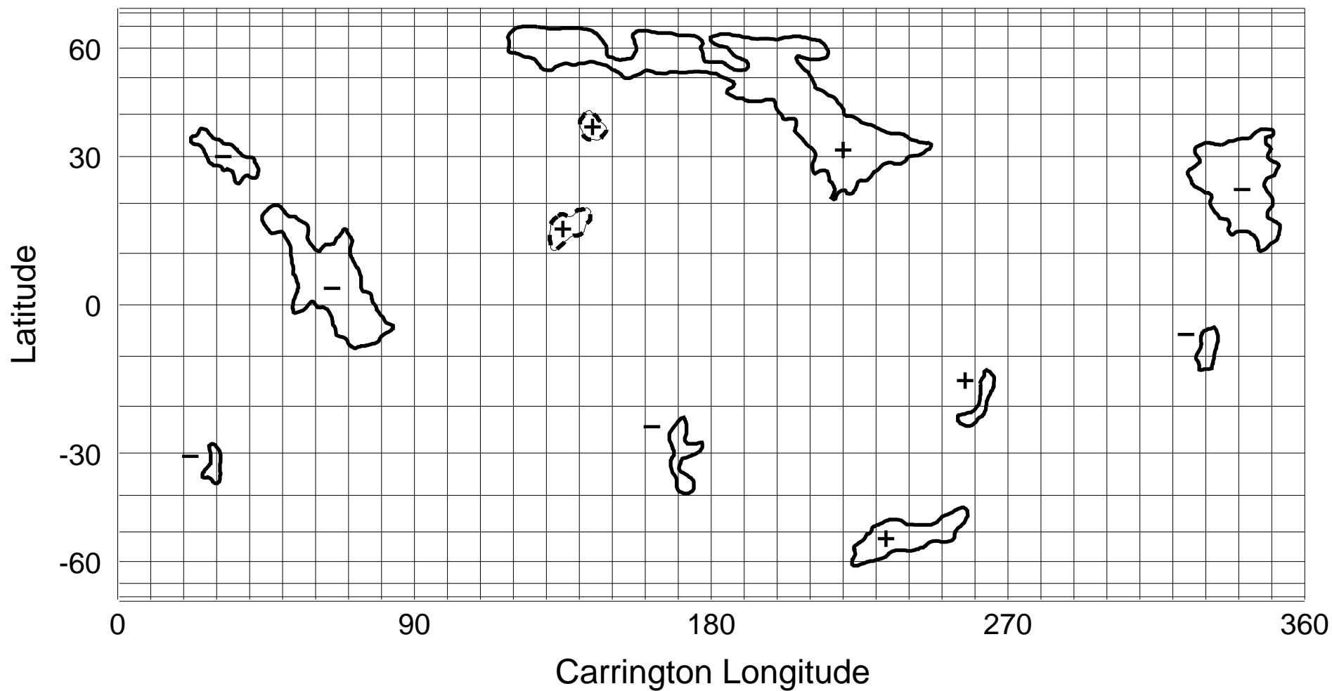
NSO/KP He I 1083 nm Coronal Hole Map: Carrington Rotation 1834
