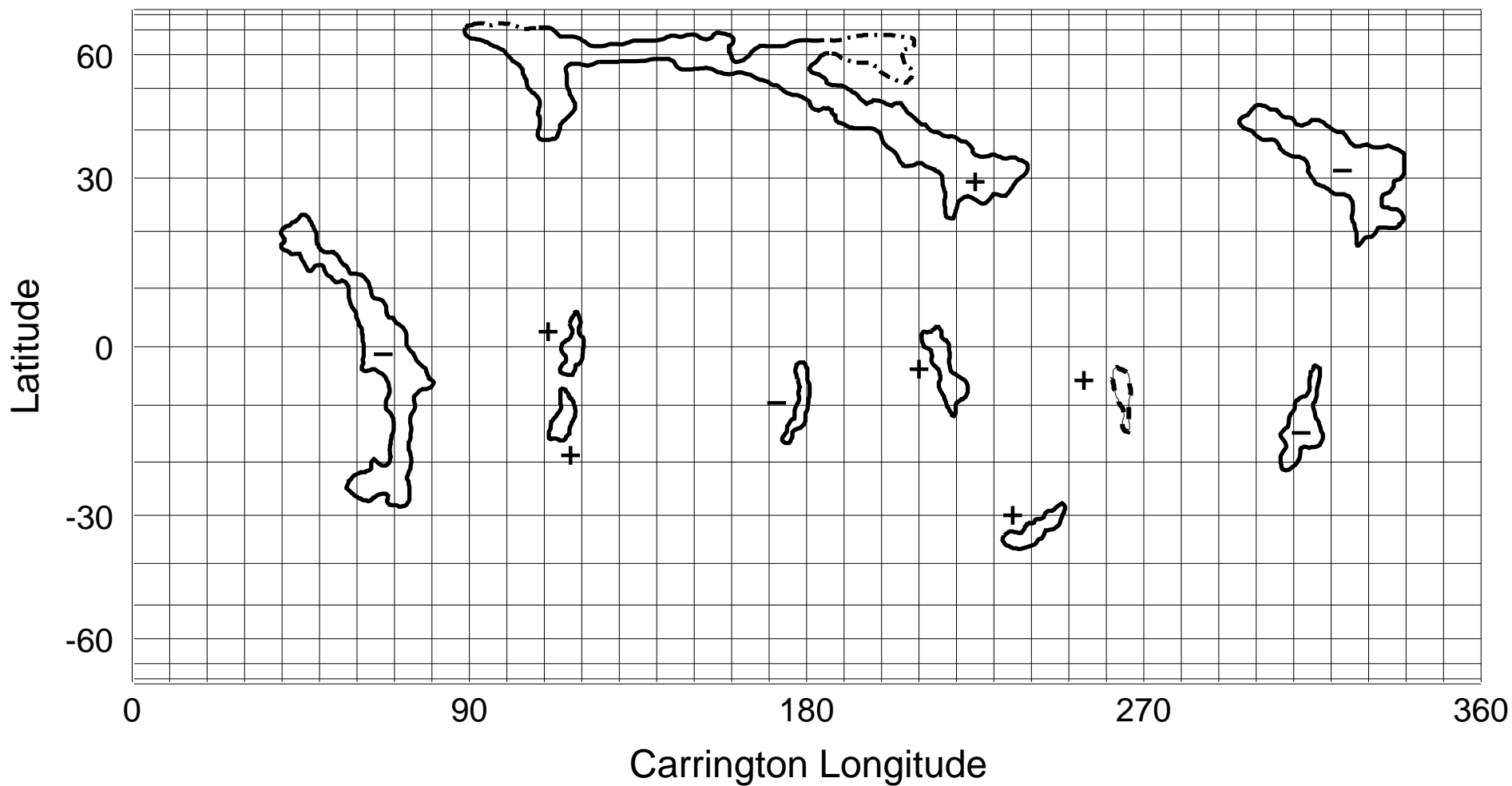
NSO/KP He I 1083 nm Coronal Hole Map: Carrington Rotation 1835
