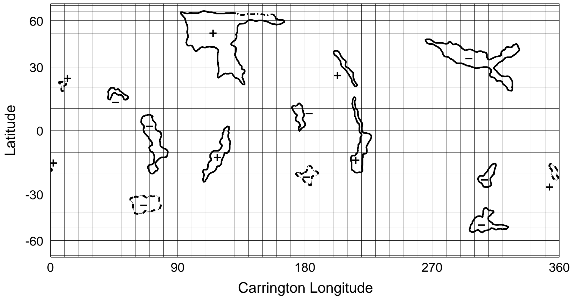
NSO/KP He I 1083 nm Coronal Hole Map: Carrington Rotation 1836
