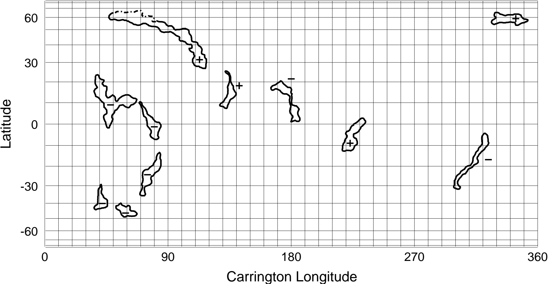
NSO/KP He I 1083 nm Coronal Hole Map: Carrington Rotation 1838
