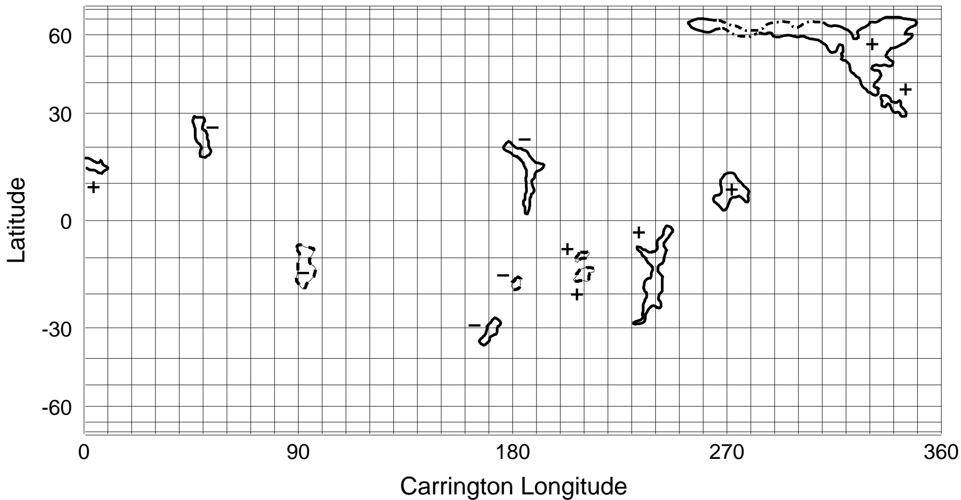
NSO/KP He I 1083 nm Coronal Hole Map: Carrington Rotation 1840
