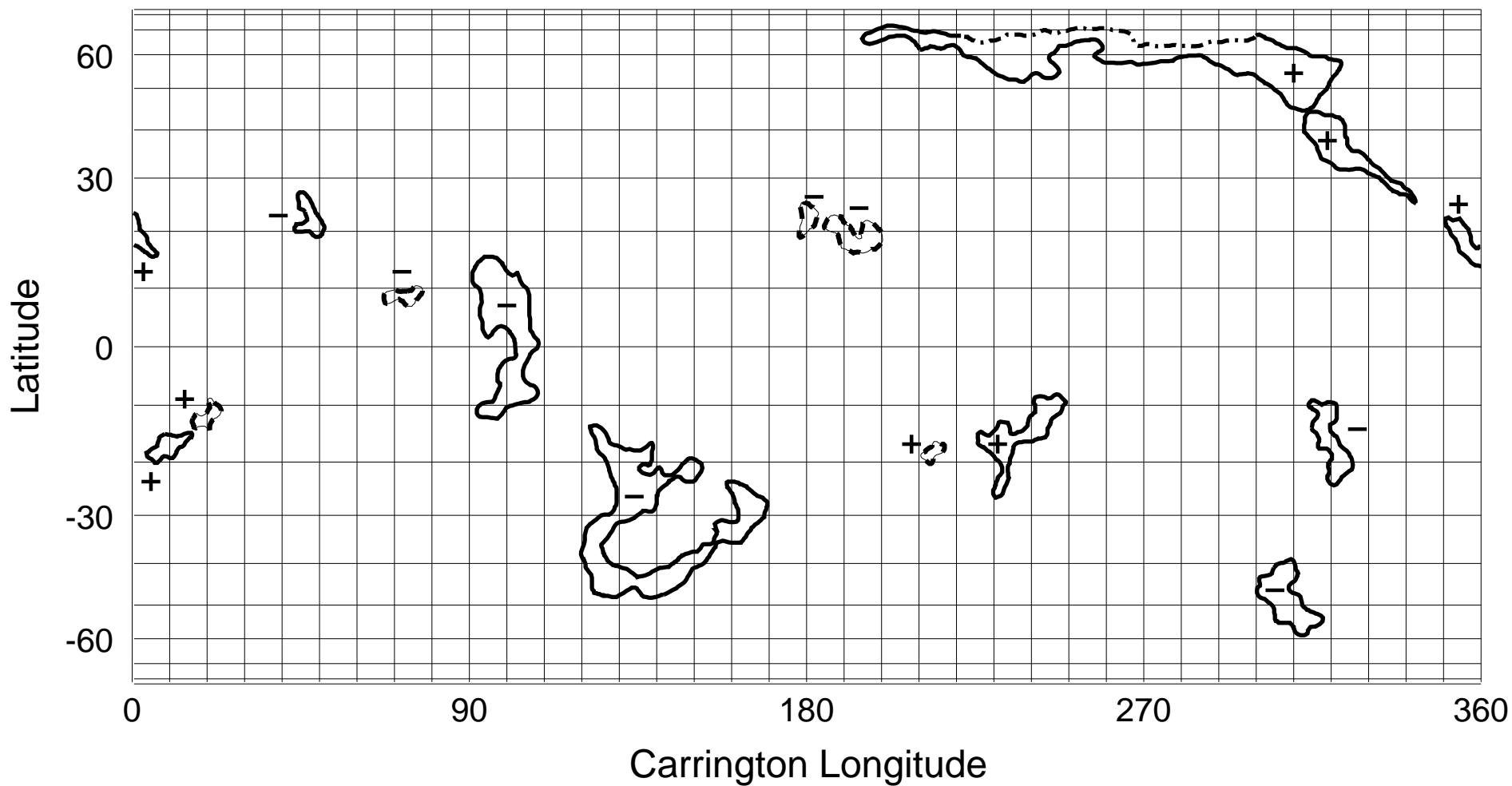
NSO/KP He I 1083 nm Coronal Hole Map: Carrington Rotation 1841
