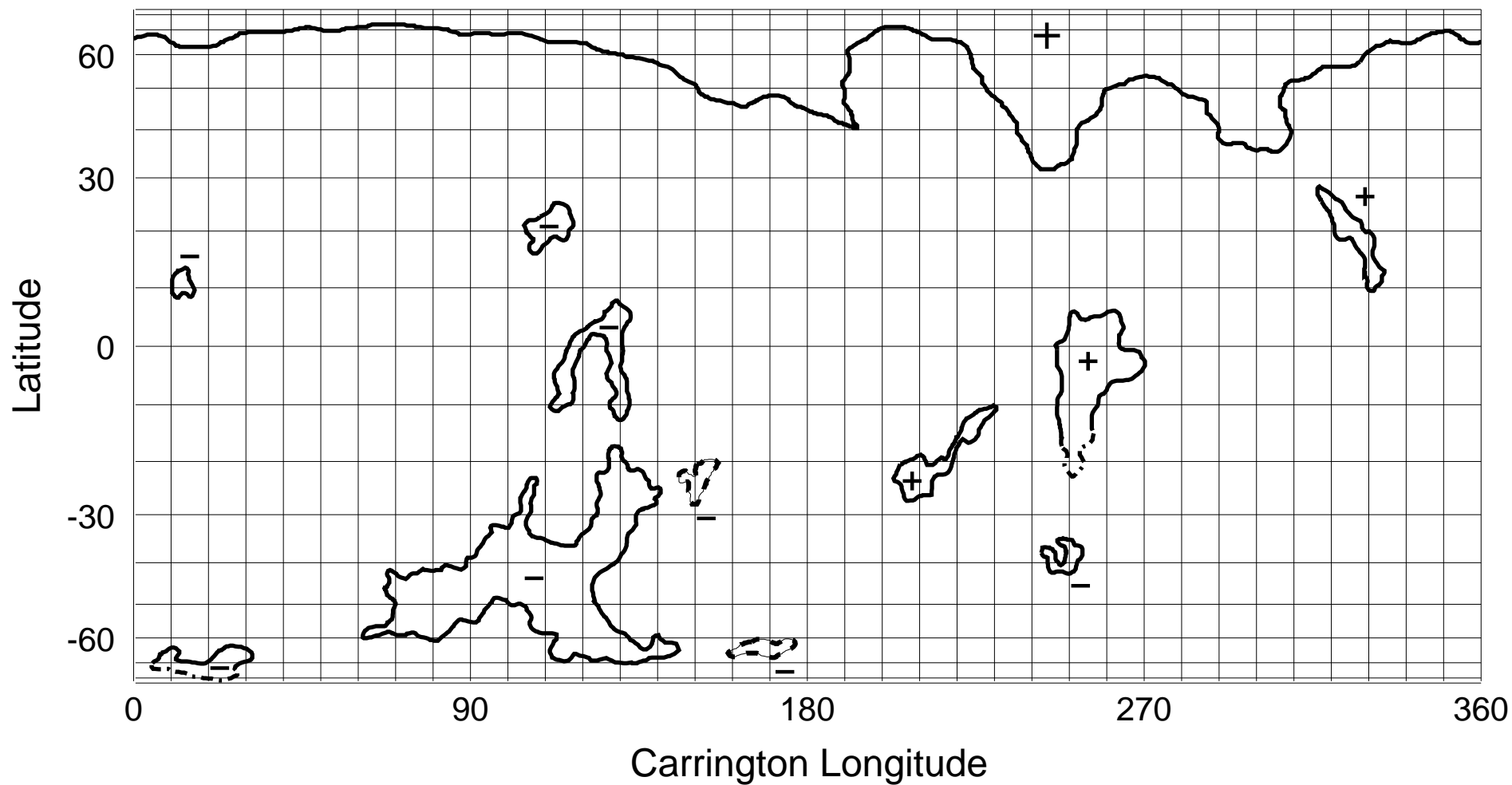
NSO/KP He I 1083 nm Coronal Hole Map: Carrington Rotation 1845
