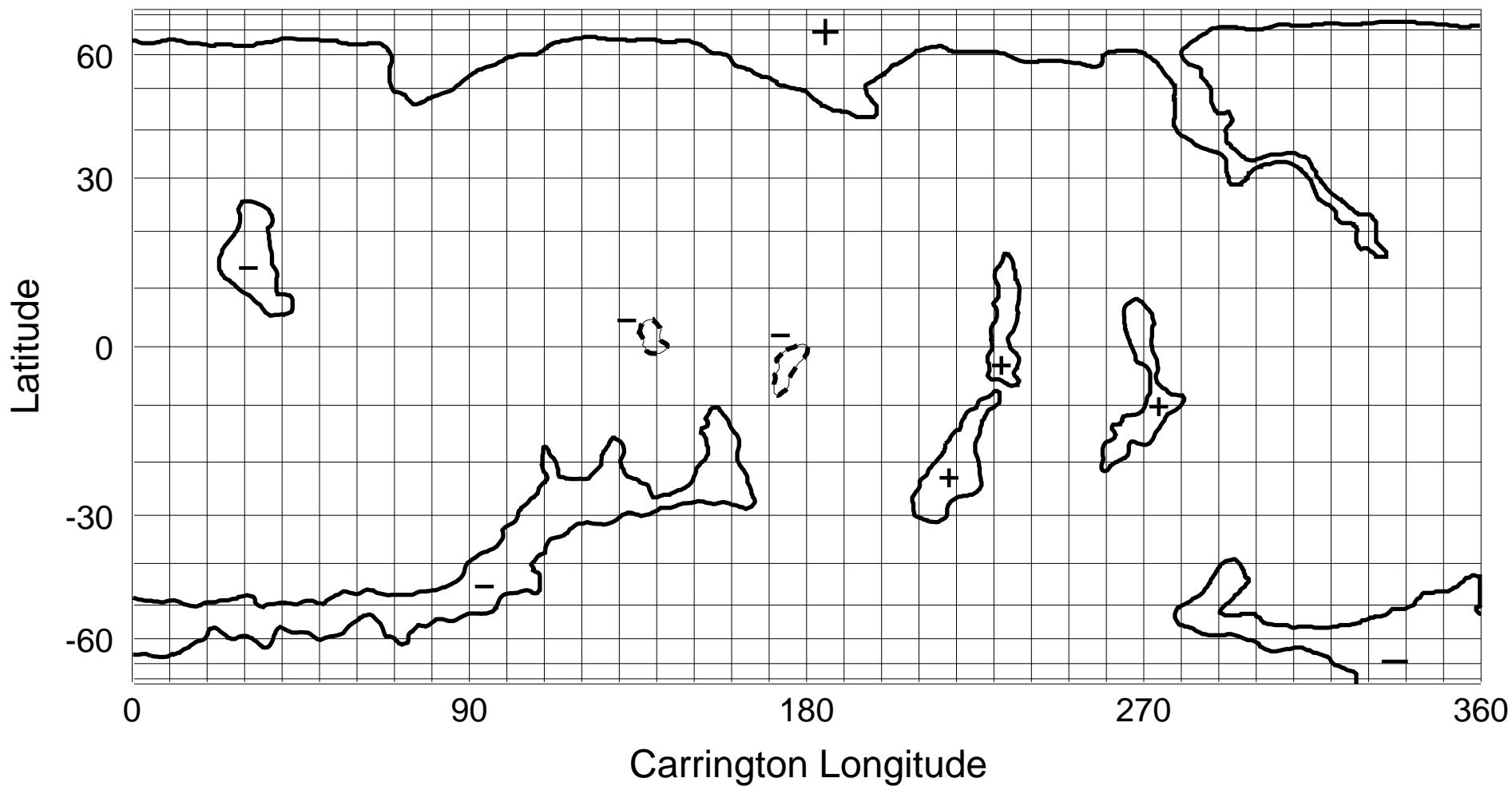
NSO/KP He I 1083 nm Coronal Hole Map: Carrington Rotation 1848
