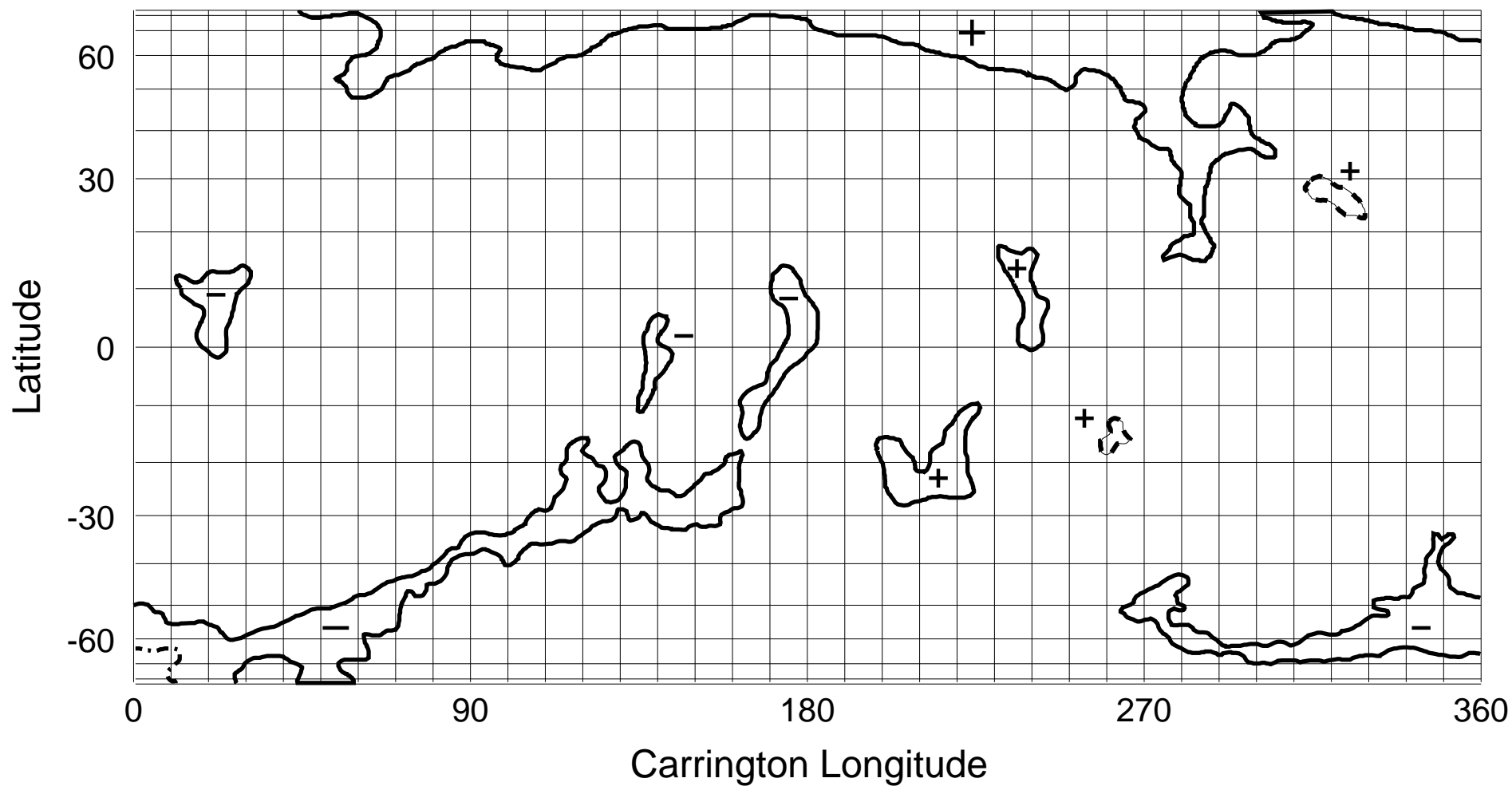
NSO/KP He I 1083 nm Coronal Hole Map: Carrington Rotation 1849
