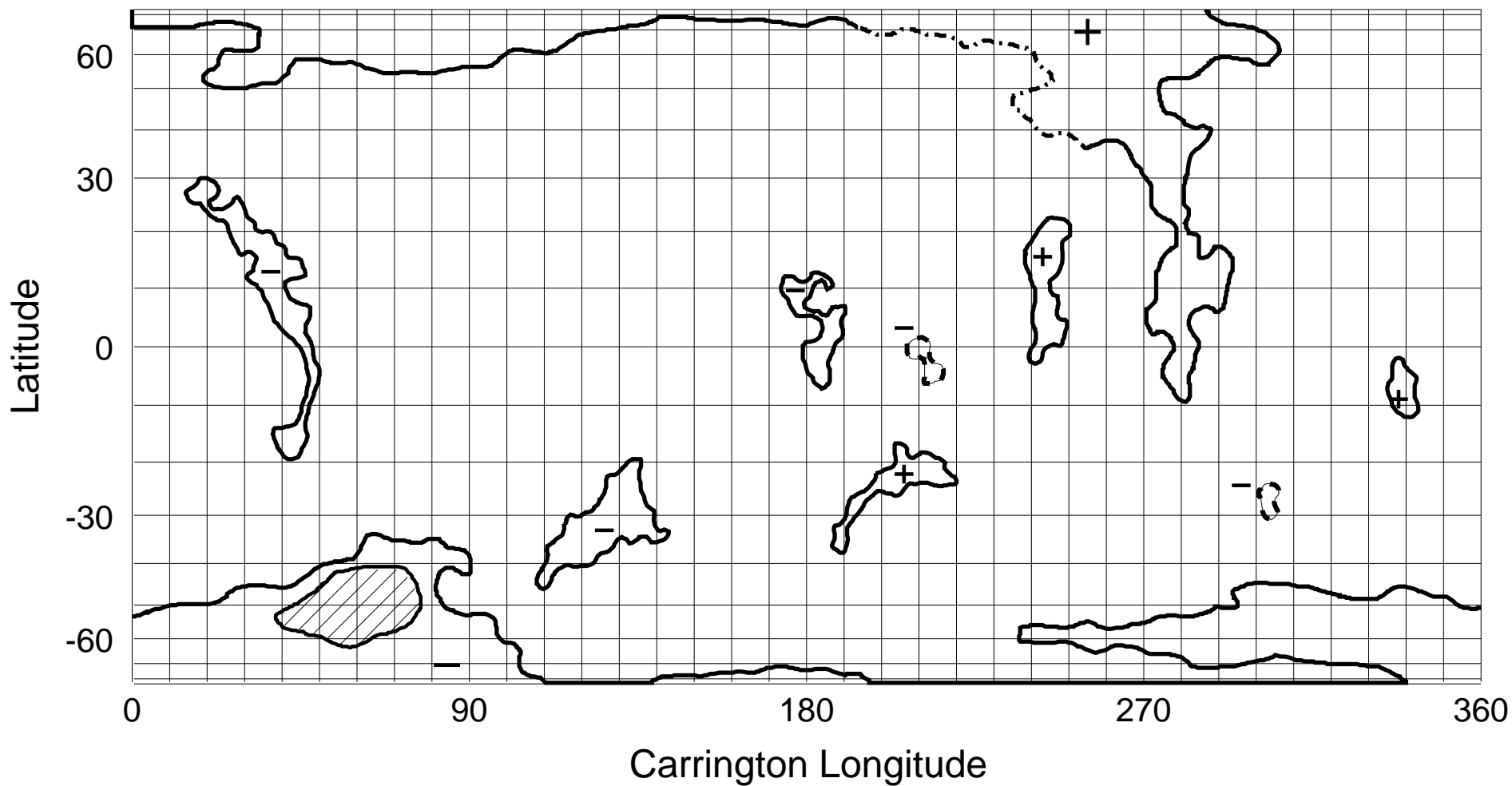
NSO/KP He I 1083 nm Coronal Hole Map: Carrington Rotation 1850
