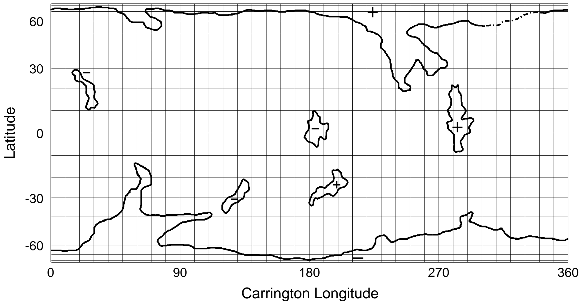
NSO/KP He I 1083 nm Coronal Hole Map: Carrington Rotation 1851
