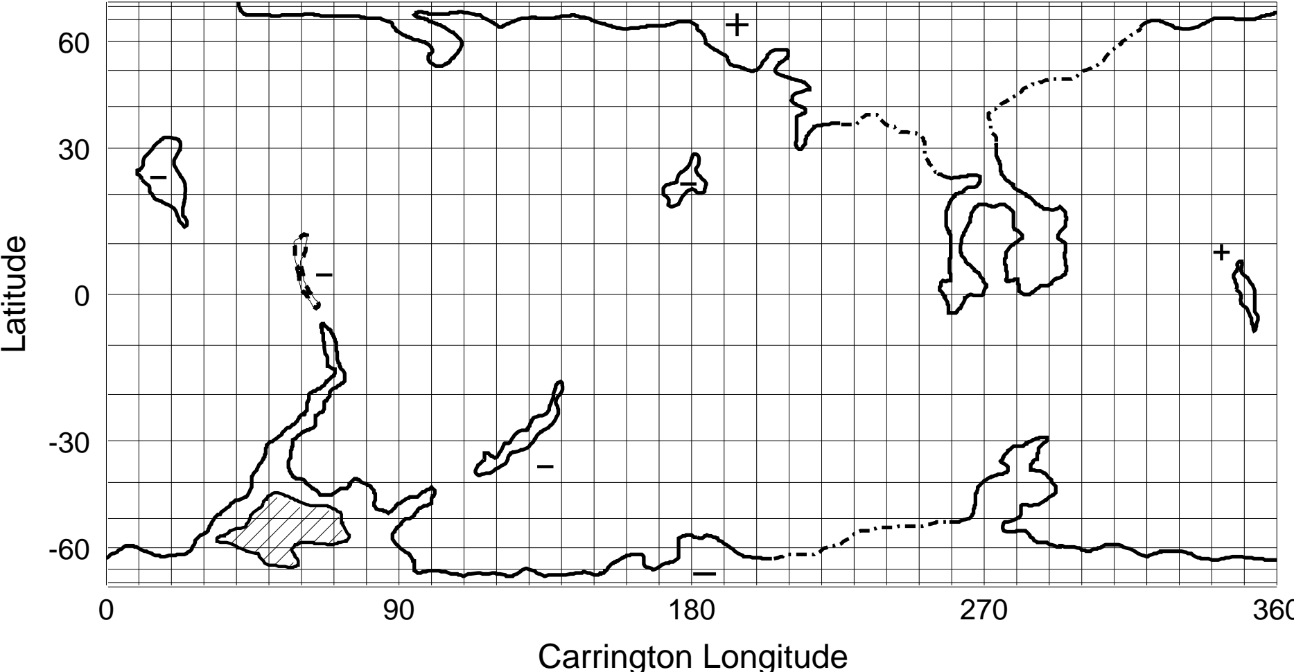
NSO/KP He I 1083 nm Coronal Hole Map: Carrington Rotation 1852
