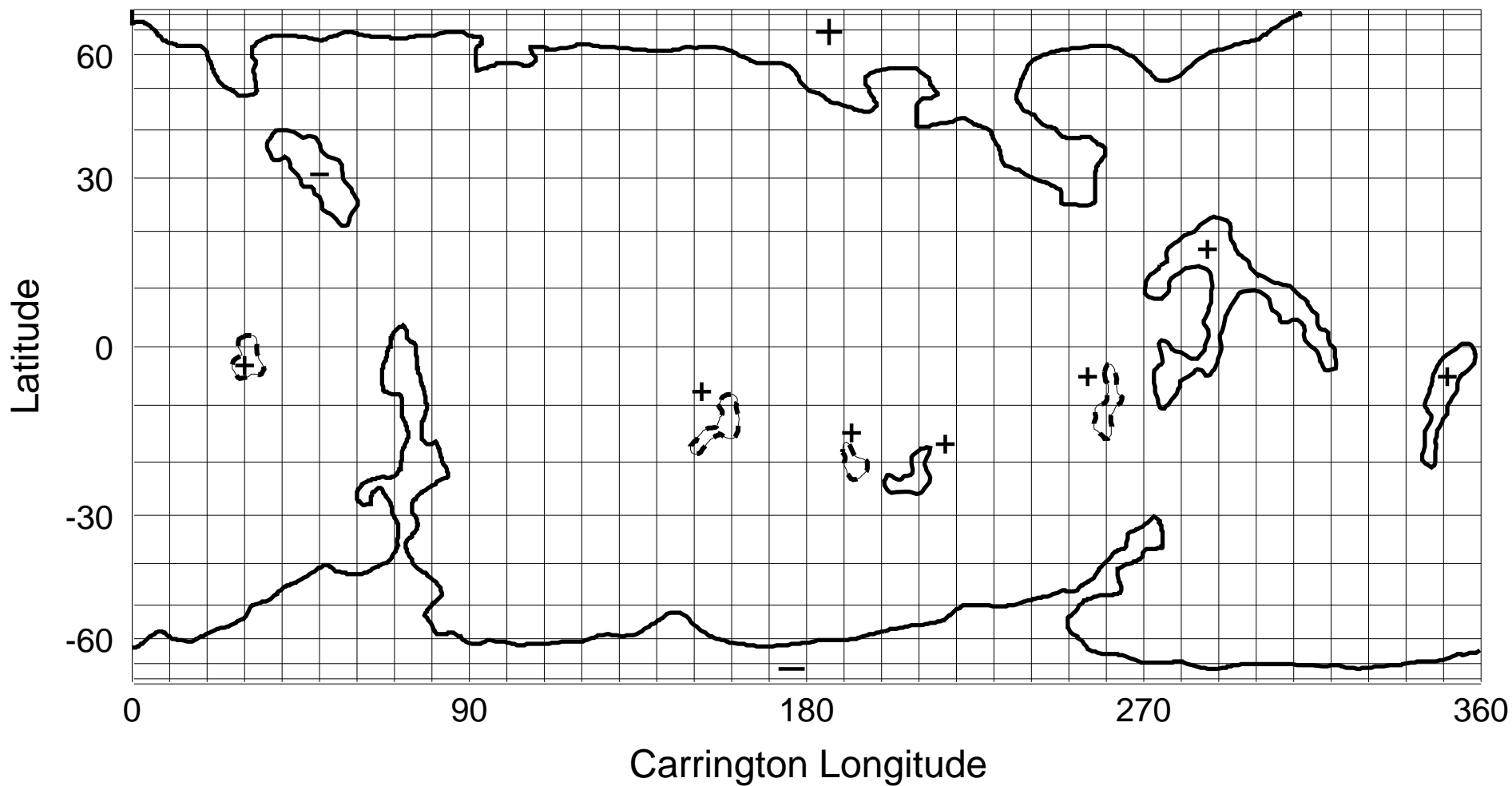
NSO/KP He I 1083 nm Coronal Hole Map: Carrington Rotation 1853
