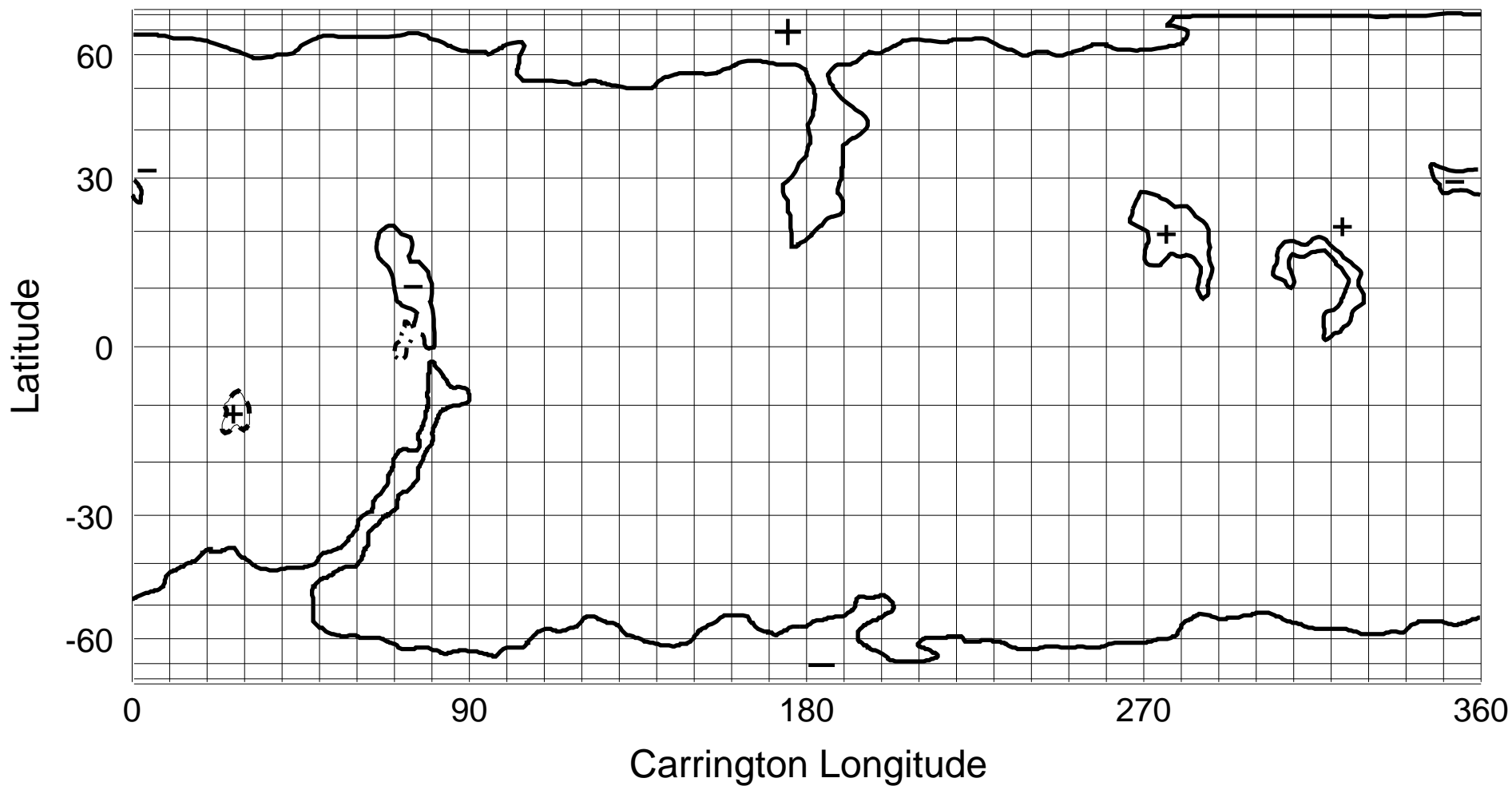
NSO/KP He I 1083 nm Coronal Hole Map: Carrington Rotation 1855
