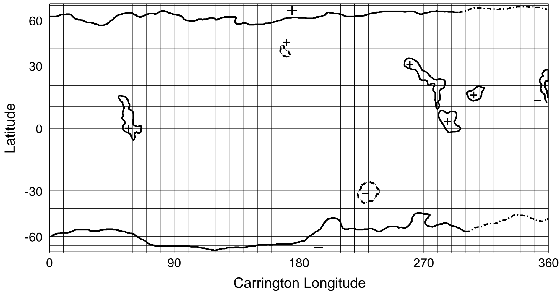
NSO/KP He I 1083 nm Coronal Hole Map: Carrington Rotation 1857
