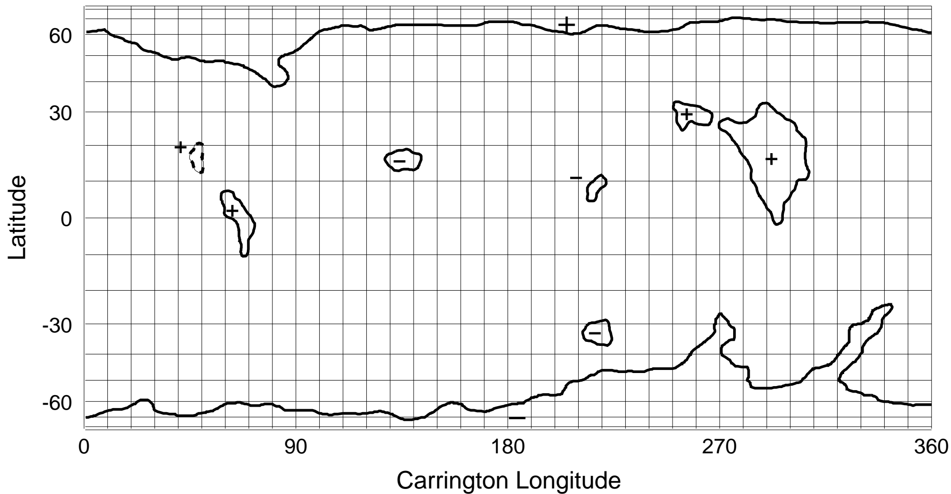
NSO/KP He I 1083 nm Coronal Hole Map: Carrington Rotation 1858
