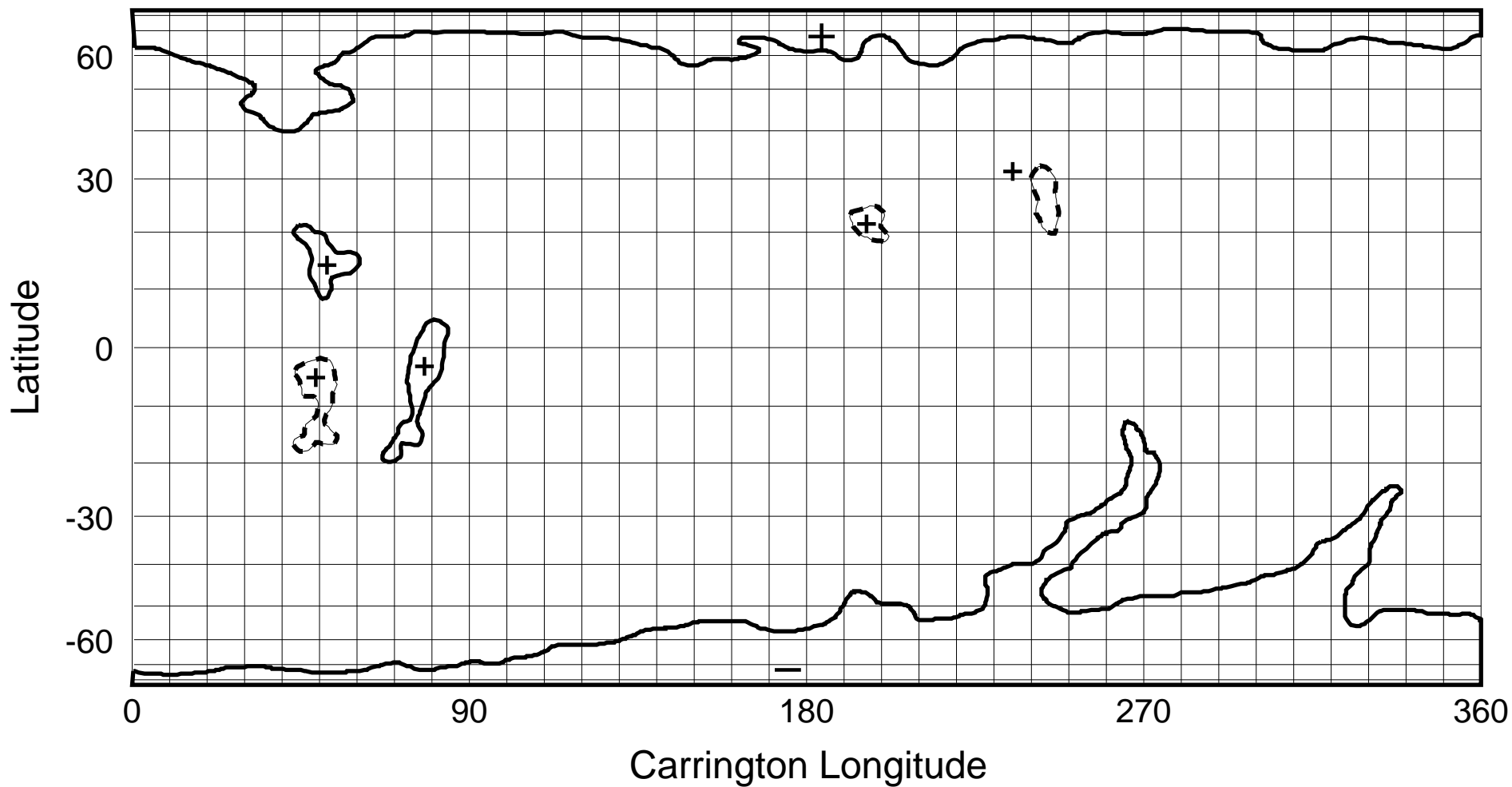
NSO/KP He I 1083 nm Coronal Hole Map: Carrington Rotation 1859
