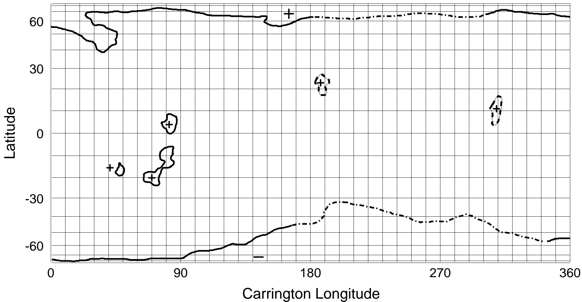
NSO/KP He I 1083 nm Coronal Hole Map: Carrington Rotation 1860
