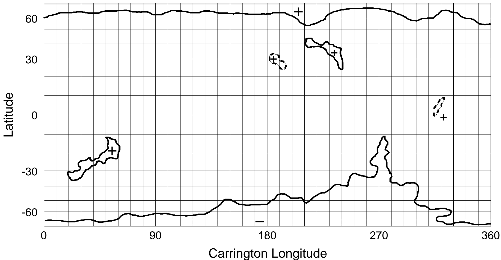
NSO/KP He I 1083 nm Coronal Hole Map: Carrington Rotation 1861
