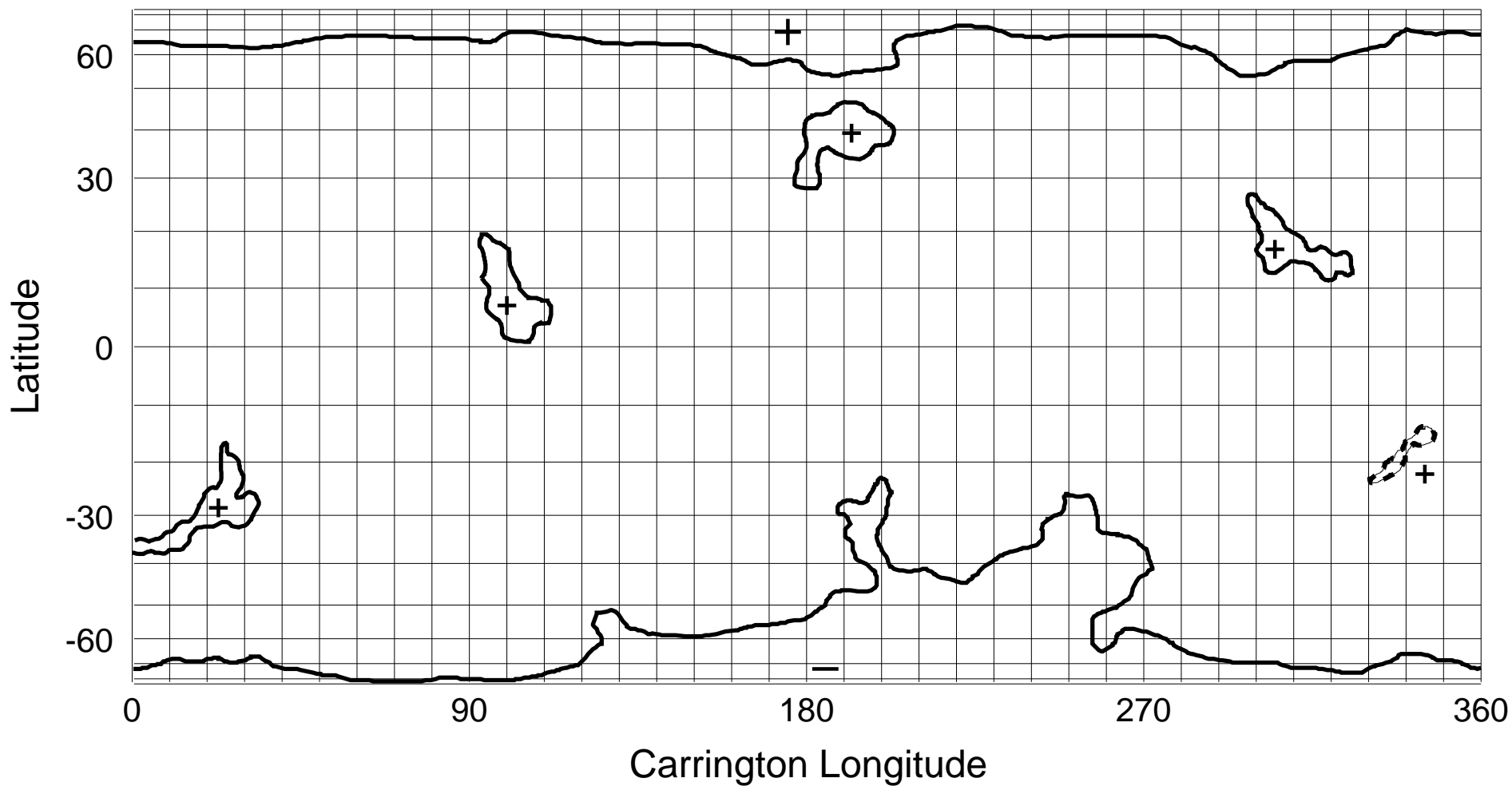
NSO/KP He I 1083 nm Coronal Hole Map: Carrington Rotation 1862
