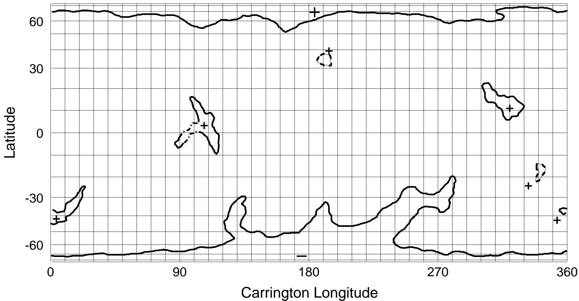
NSO/KP He I 1083 nm Coronal Hole Map: Carrington Rotation 1863
