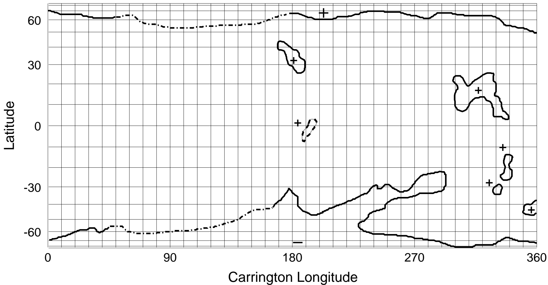
NSO/KP He I 1083 nm Coronal Hole Map: Carrington Rotation 1864
