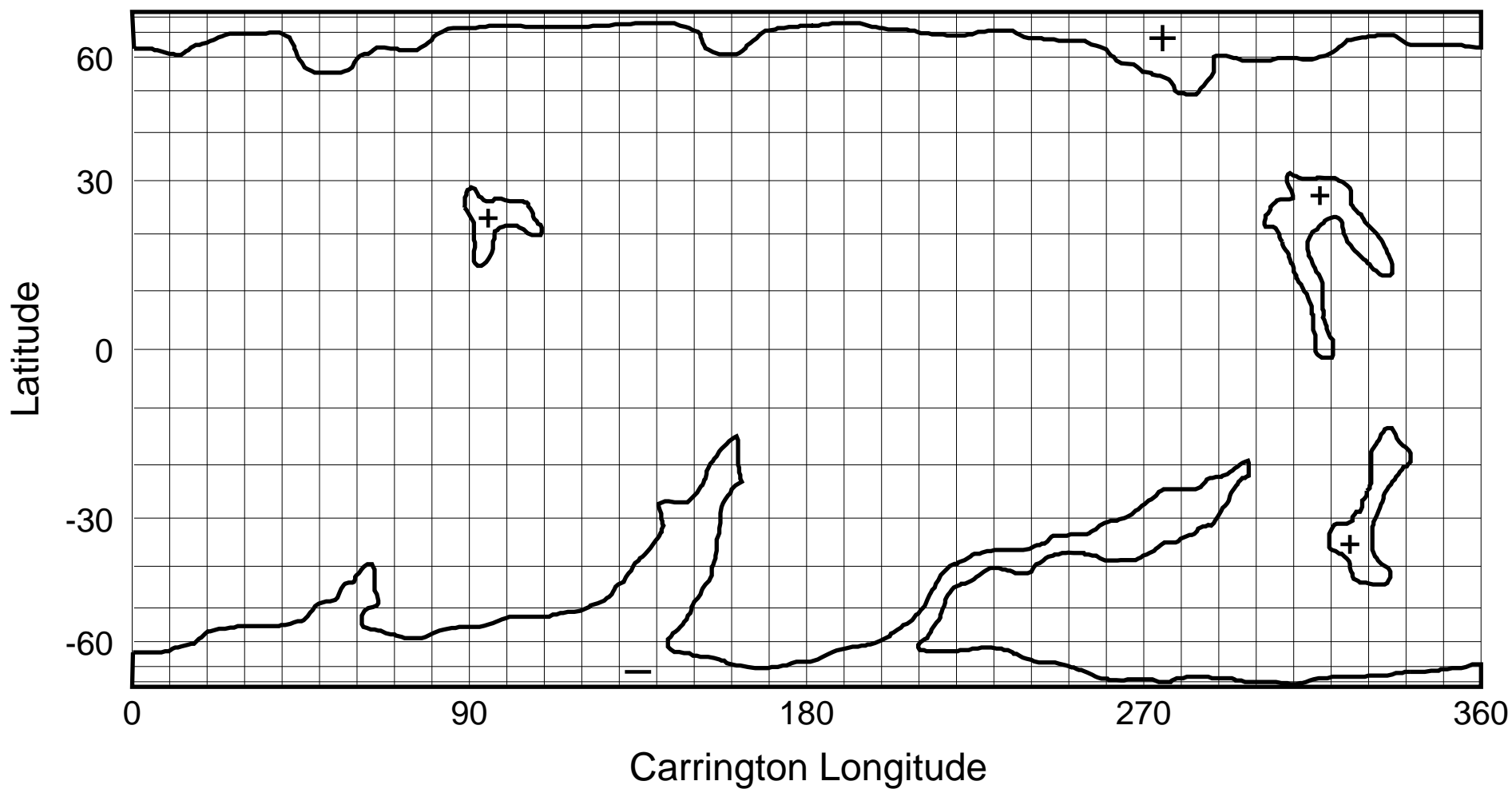
NSO/KP He I 1083 nm Coronal Hole Map: Carrington Rotation 1865
