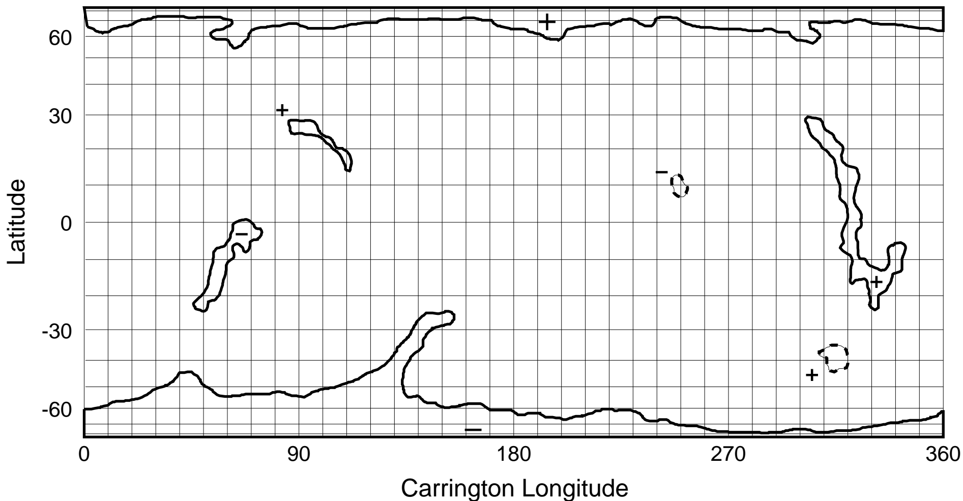
NSO/KP He I 1083 nm Coronal Hole Map: Carrington Rotation 1866
