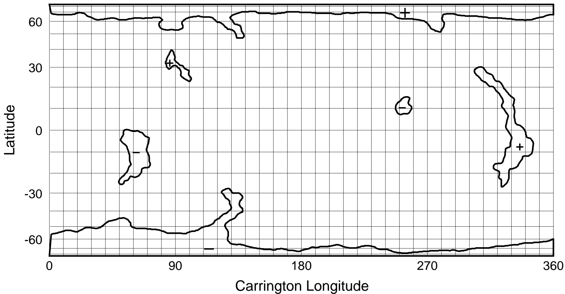
NSO/KP He I 1083 nm Coronal Hole Map: Carrington Rotation 1867
