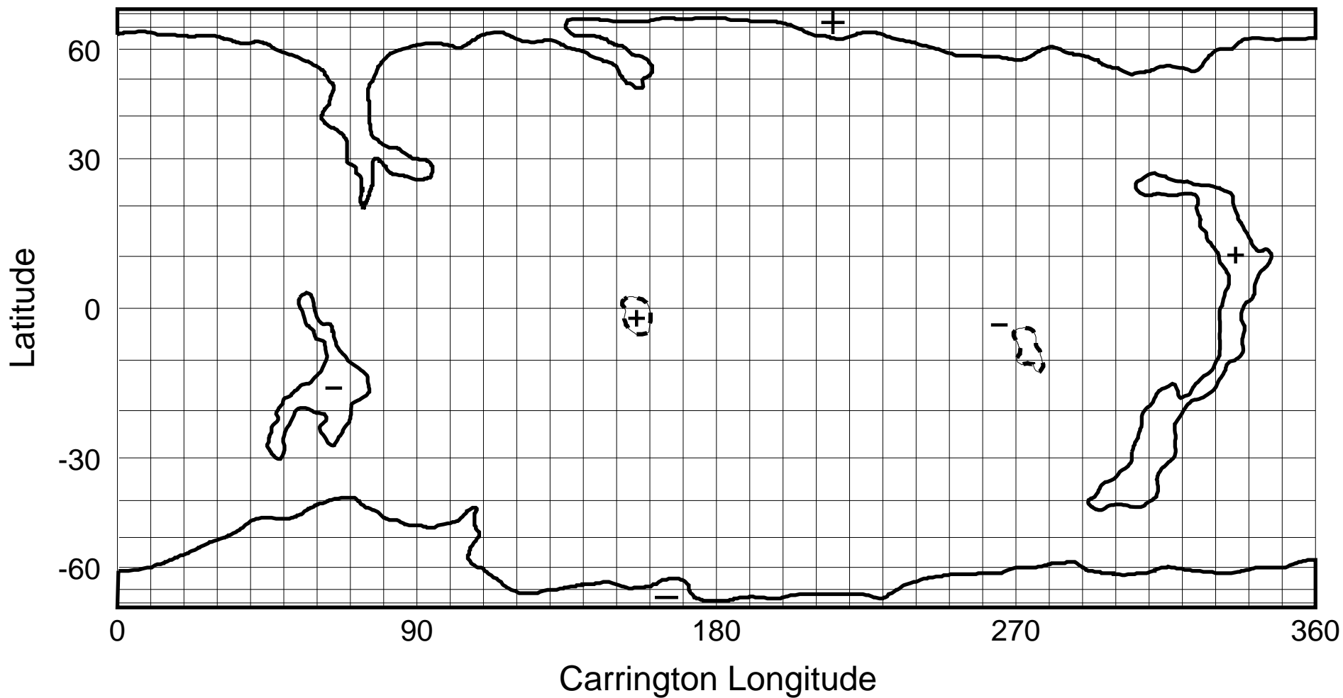
NSO/KP He I 1083 nm Coronal Hole Map: Carrington Rotation 1868
