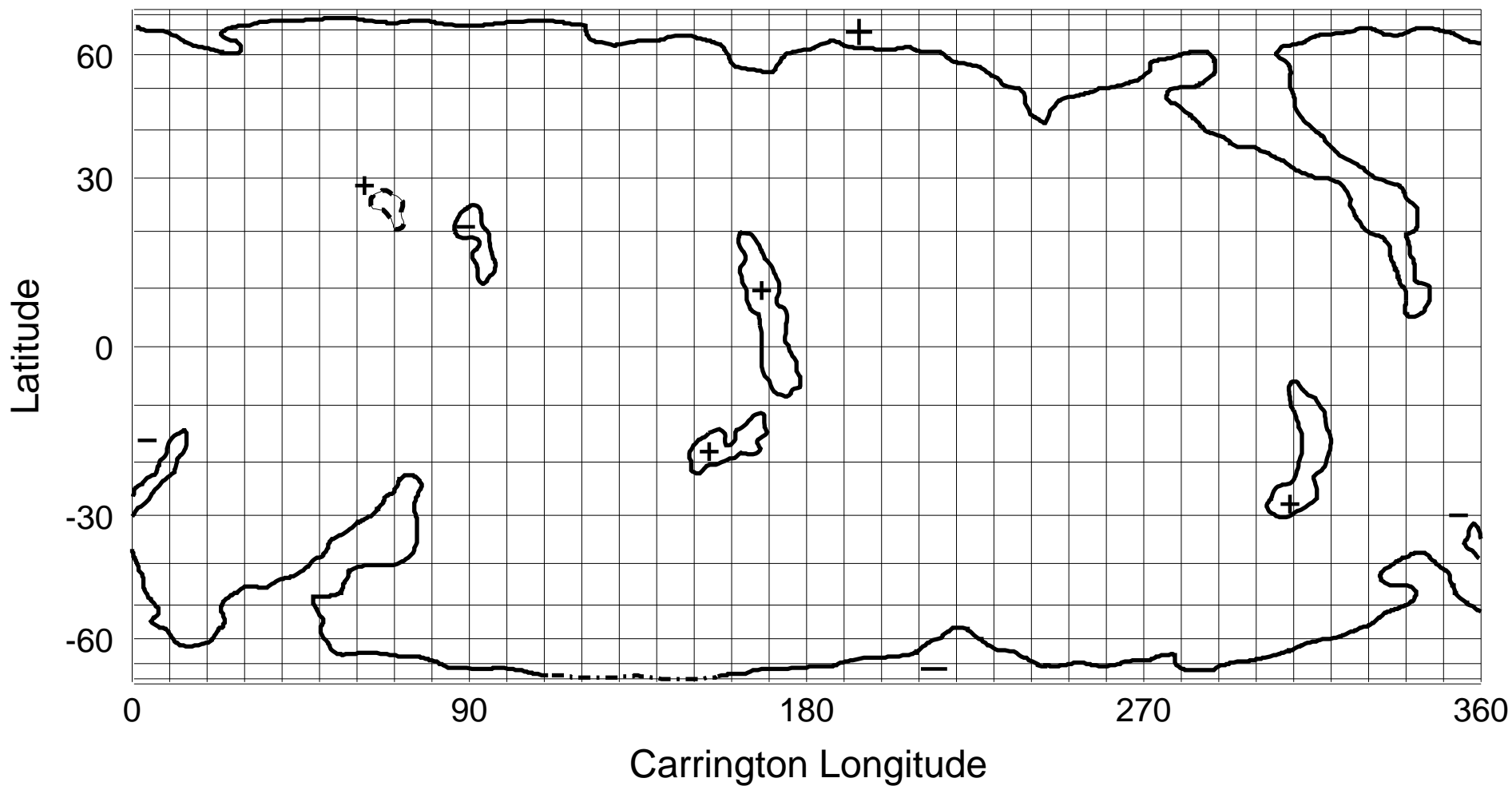
NSO/KP He I 1083 nm Coronal Hole Map: Carrington Rotation 1871
