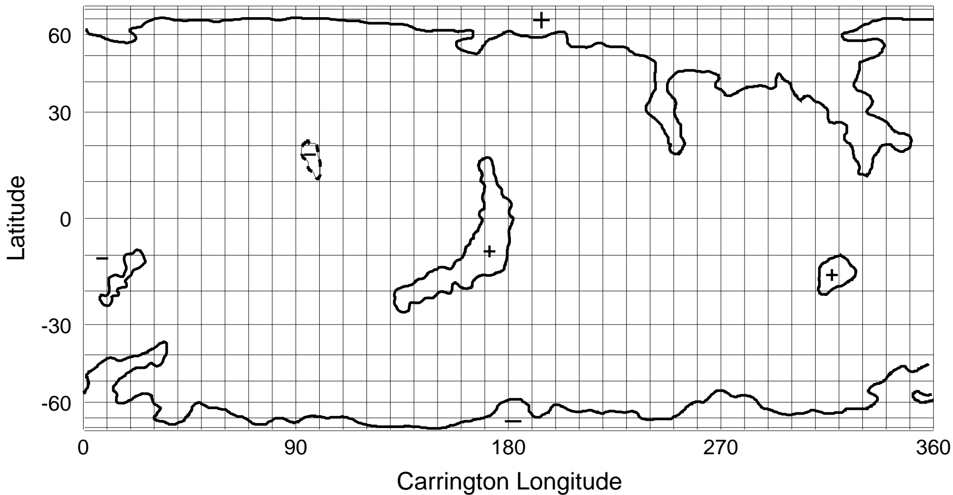
NSO/KP He I 1083 nm Coronal Hole Map: Carrington Rotation 1872
