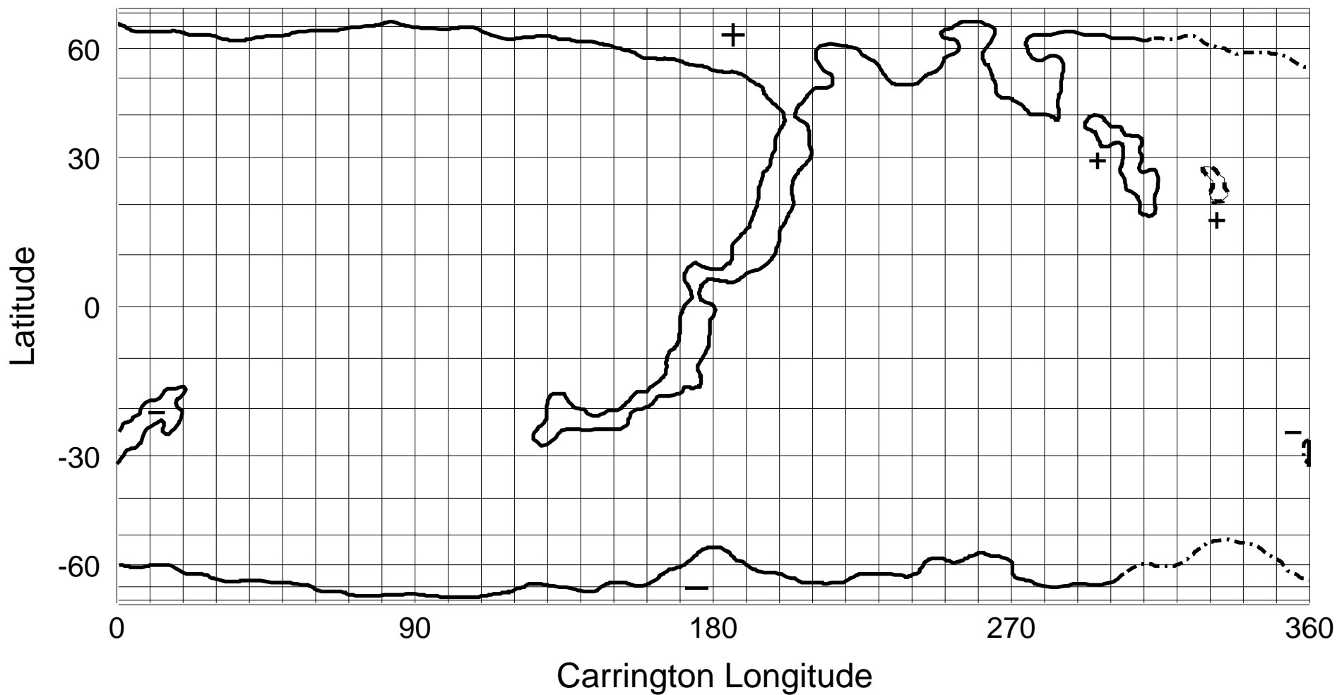
NSO/KP He I 1083 nm Coronal Hole Map: Carrington Rotation 1873
