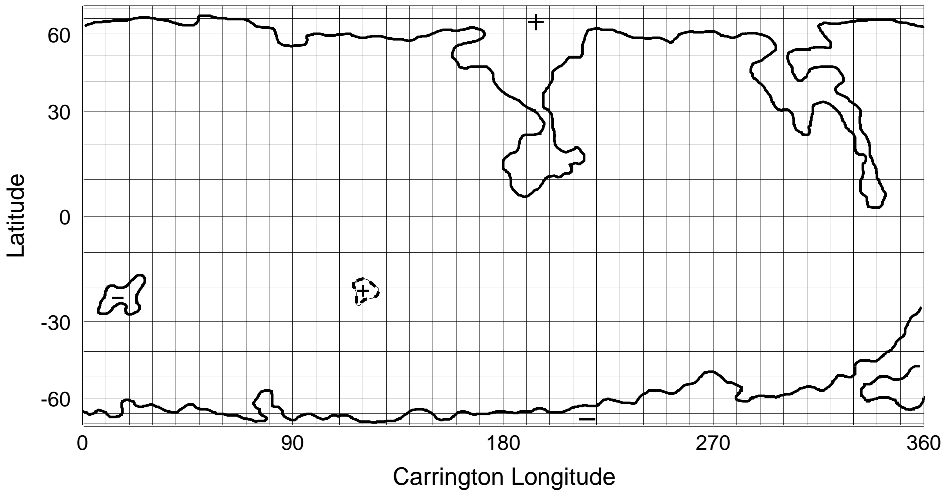
NSO/KP He I 1083 nm Coronal Hole Map: Carrington Rotation 1874
