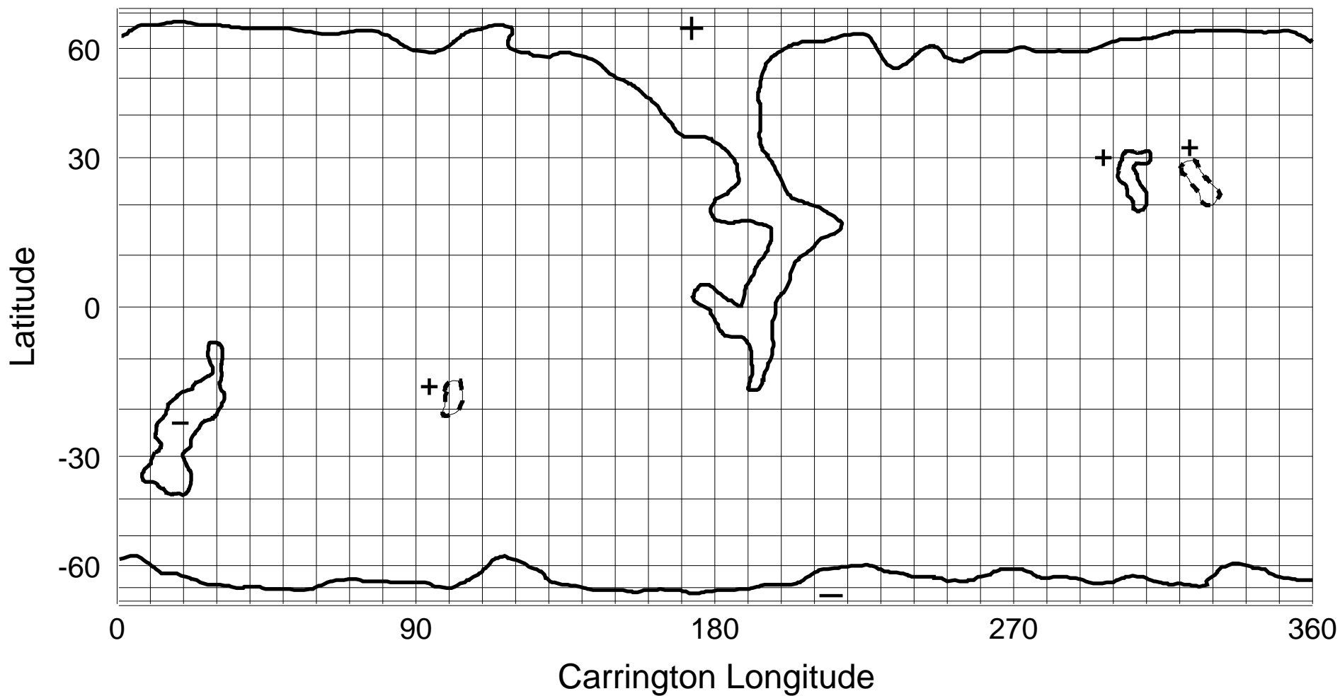
NSO/KP He I 1083 nm Coronal Hole Map: Carrington Rotation 1875
