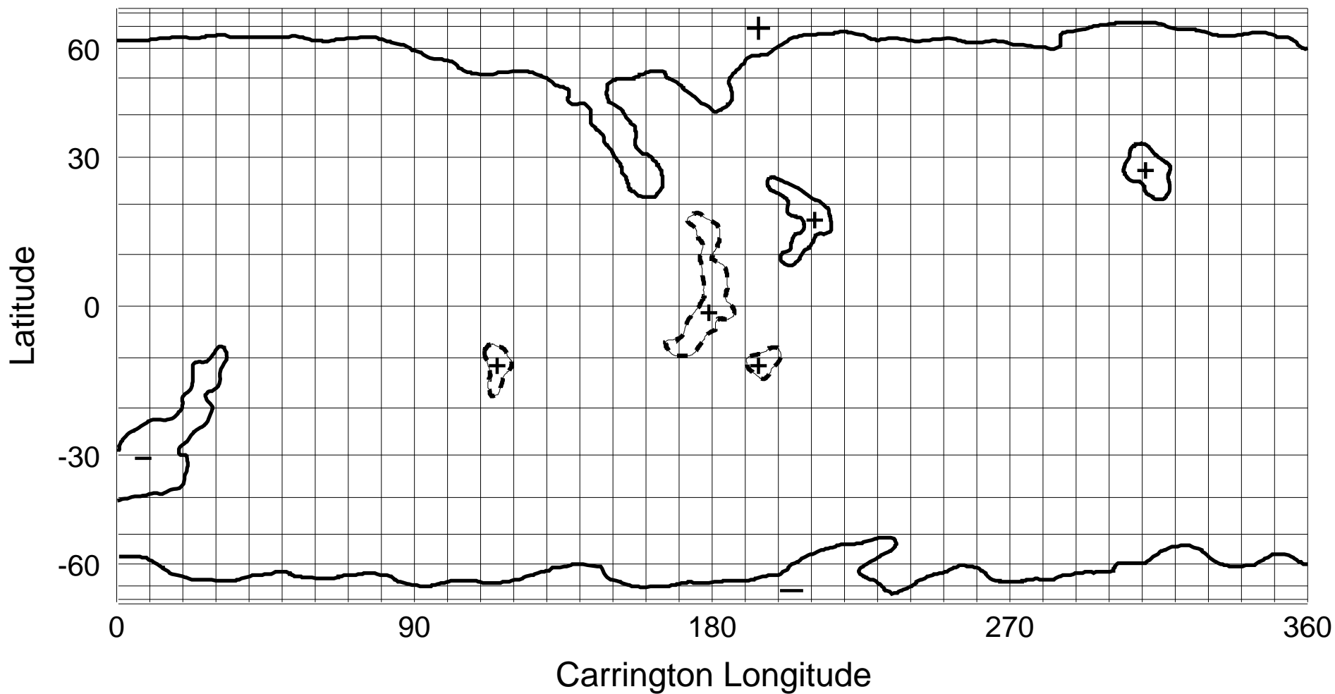
NSO/KP He I 1083 nm Coronal Hole Map: Carrington Rotation 1876
