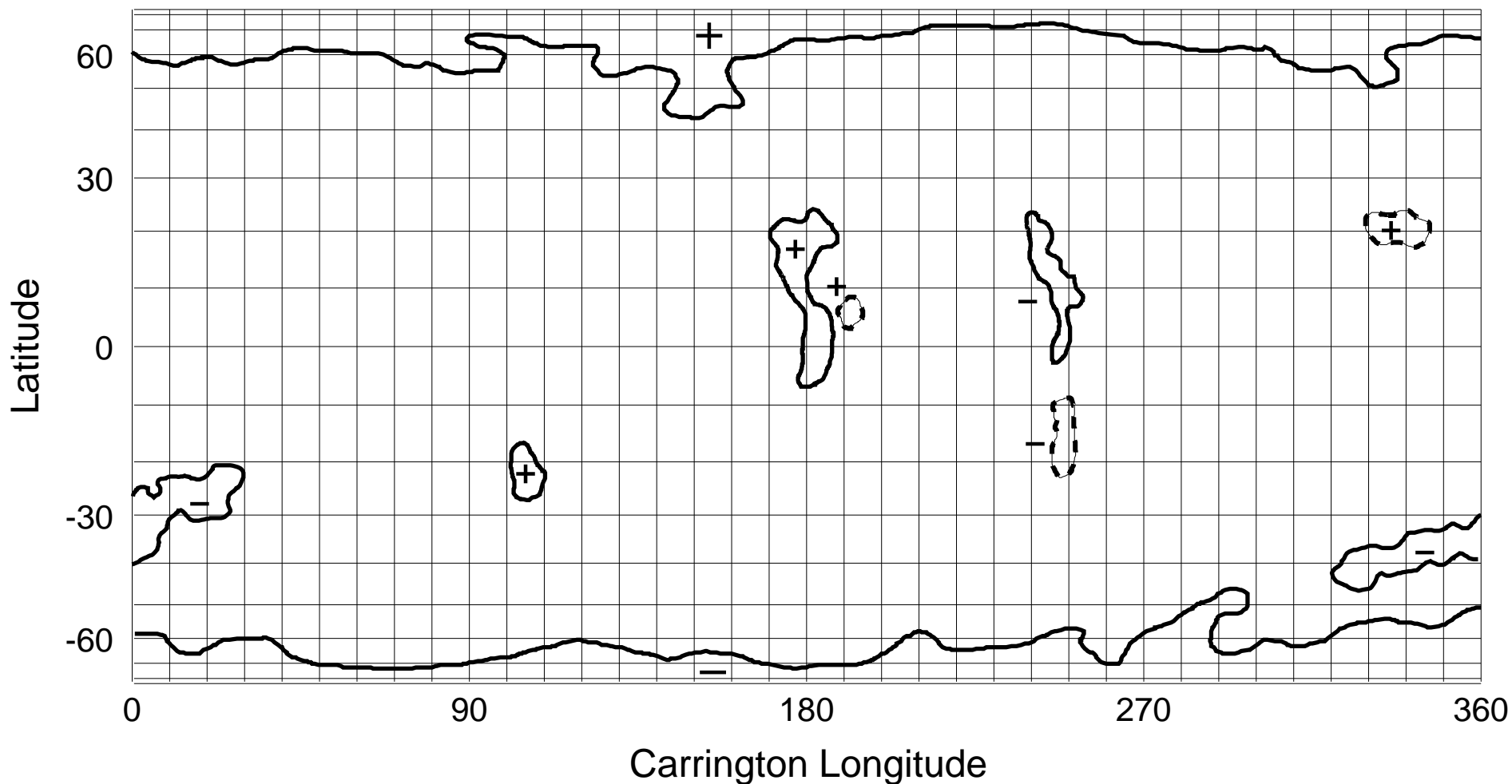
NSO/KP He I 1083 nm Coronal Hole Map: Carrington Rotation 1878
