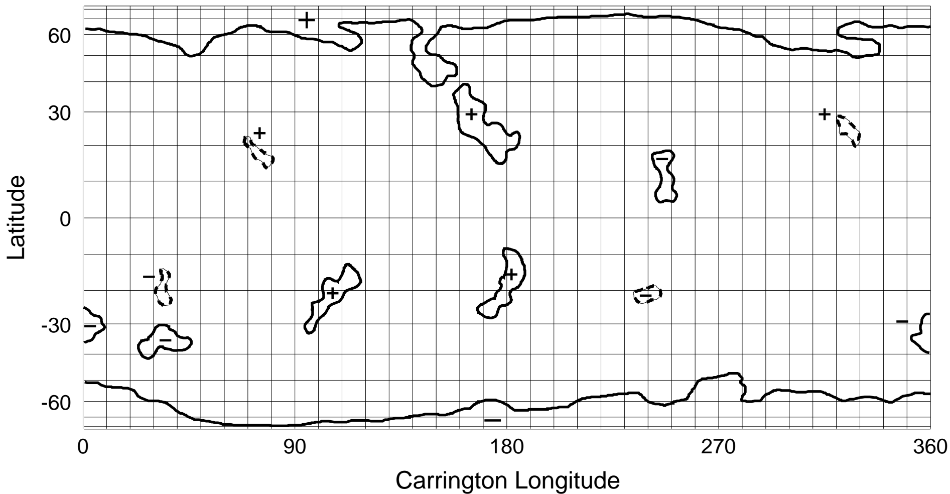
NSO/KP He I 1083 nm Coronal Hole Map: Carrington Rotation 1879
