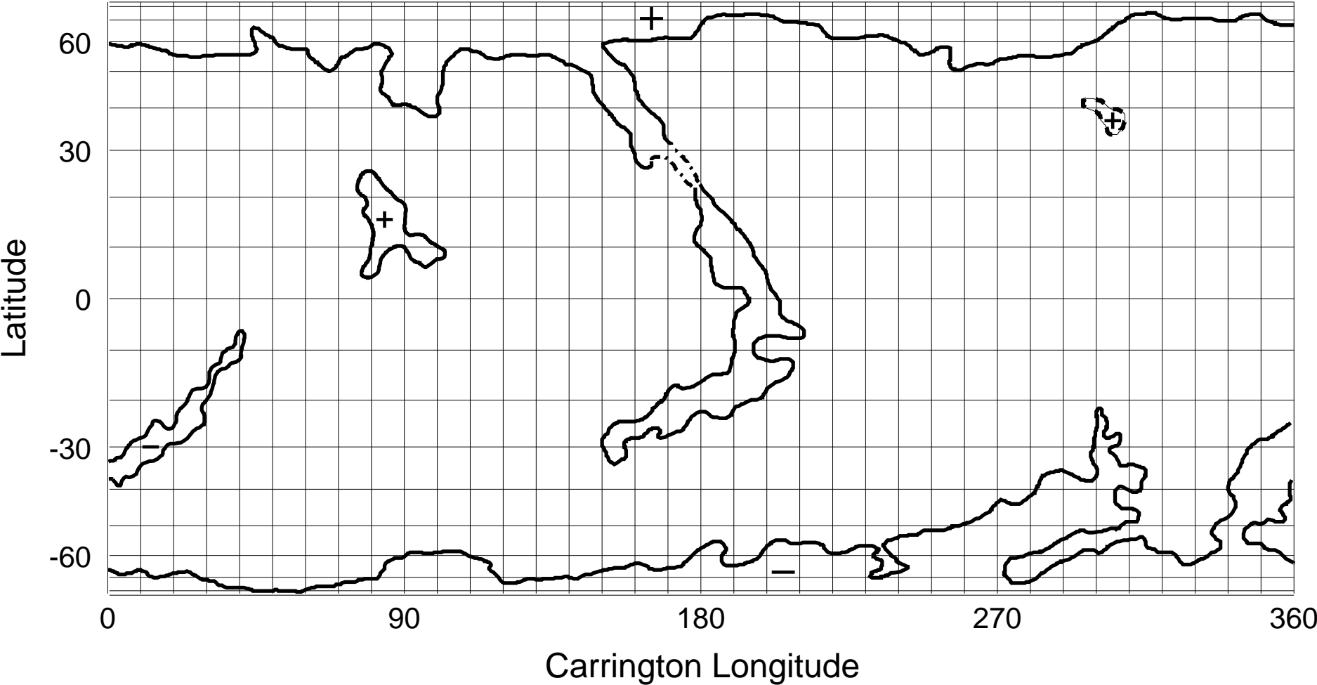
NSO/KP He I 1083 nm Coronal Hole Map: Carrington Rotation 1882
