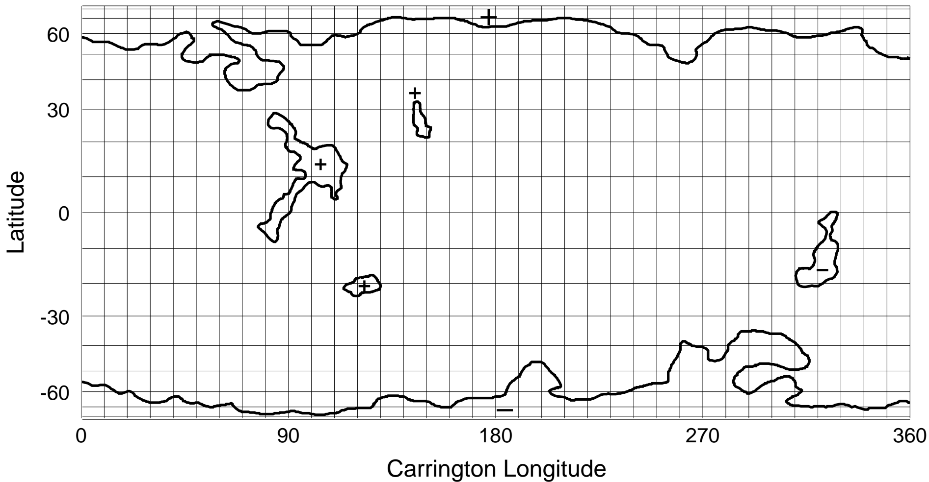
NSO/KP He I 1083 nm Coronal Hole Map: Carrington Rotation 1884
