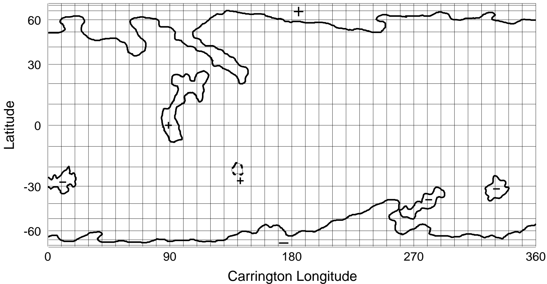
NSO/KP He I 1083 nm Coronal Hole Map: Carrington Rotation 1885
